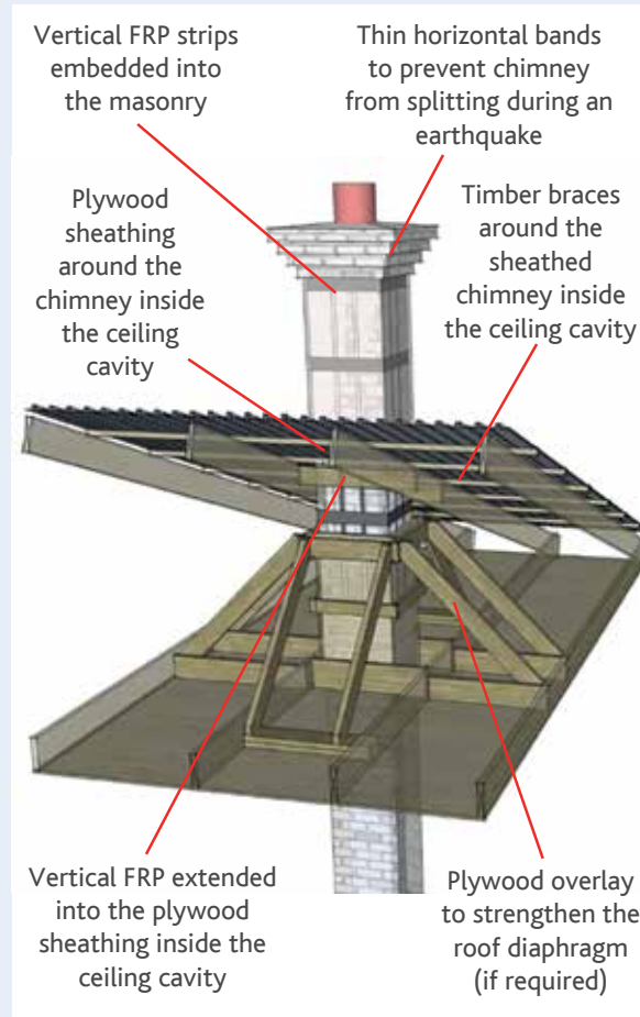
FIGURE 15: Example of FRP retrofit of URM chimneys
