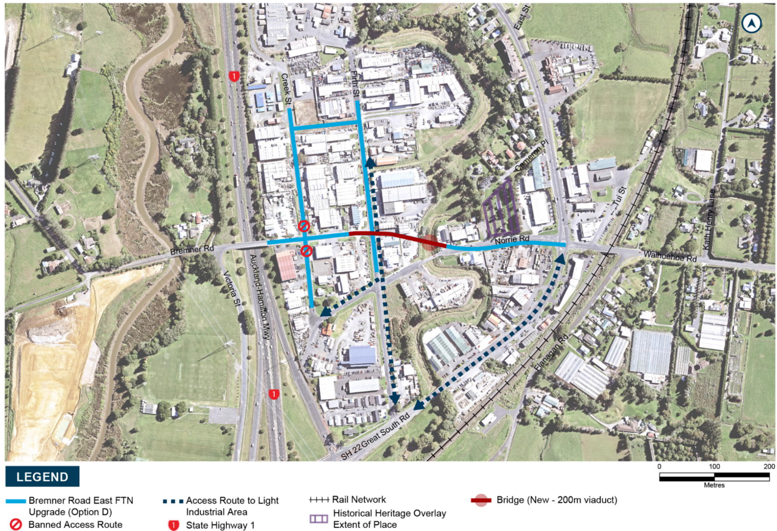
Figure 11-15: Option D – long bridge, Firth Street under
