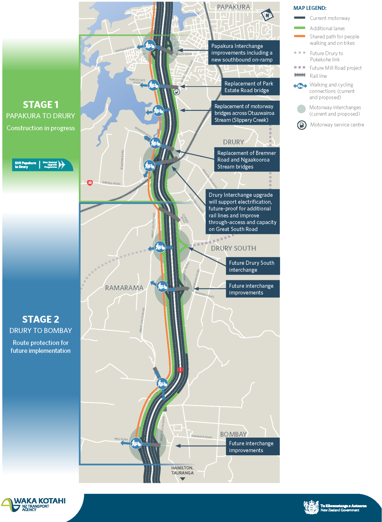
Figure 2-1: Indicative location plan showing Stage 2 of the NZTA Project
