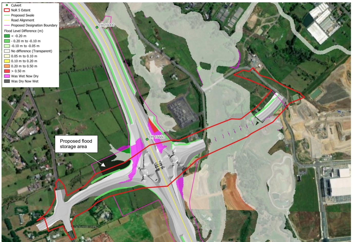
Figure 10-5 Result of sensitivity test for the 1% AEP event with climate change
