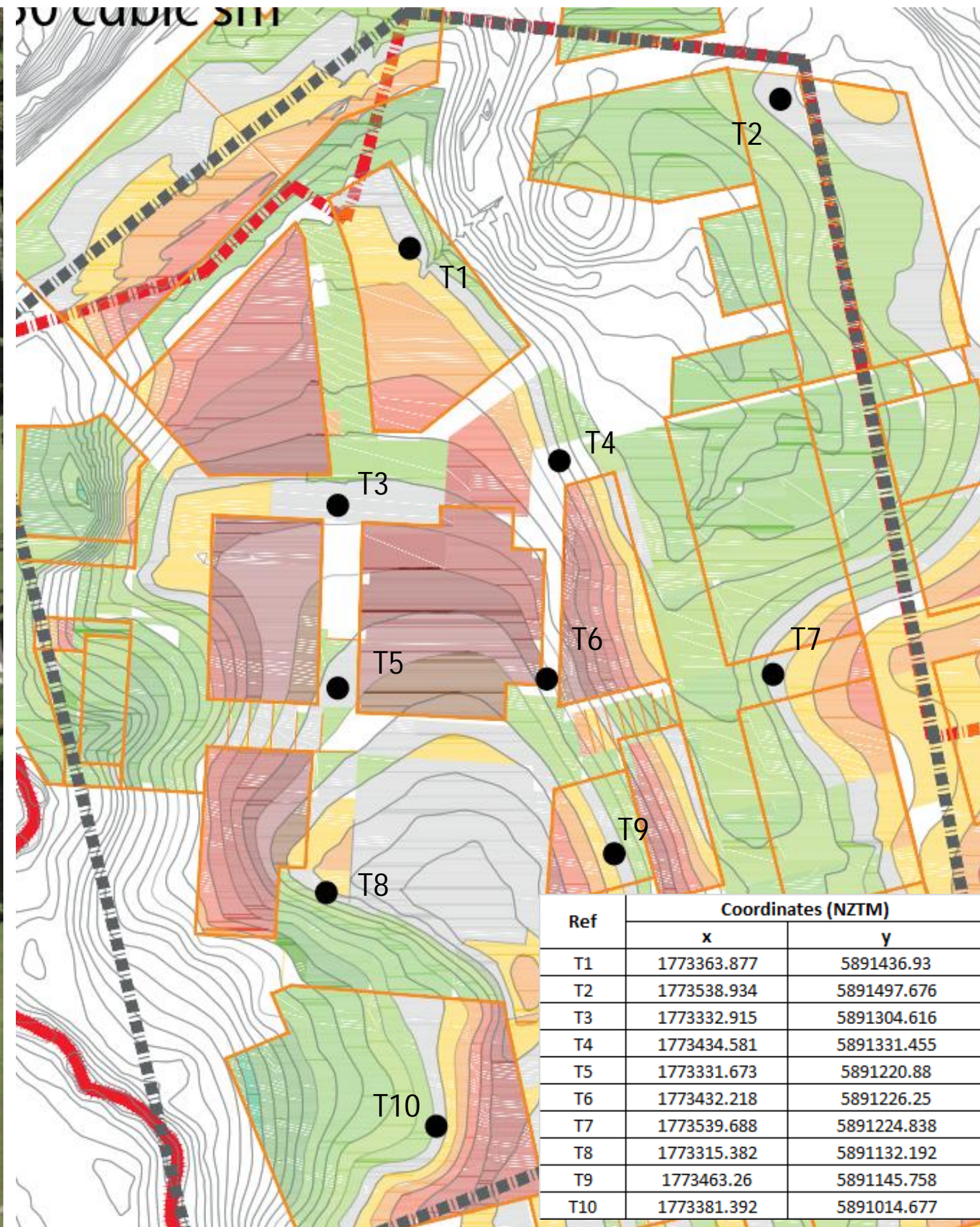
Percolation Test Location Plan provided by Tonkin and Taylor Limited via email dated 4 December 2018
