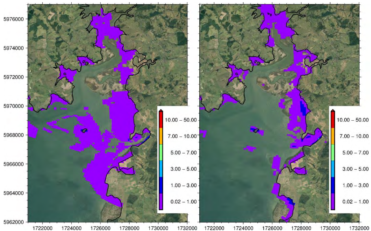
Figure 28: Additional deposition arising from Project construction at 3 days (left) and at end of 7 day simulation (right) for the 50-year ARI, calm wind event. Note: additional deposition lower than 0.02 mm are not shown here.
