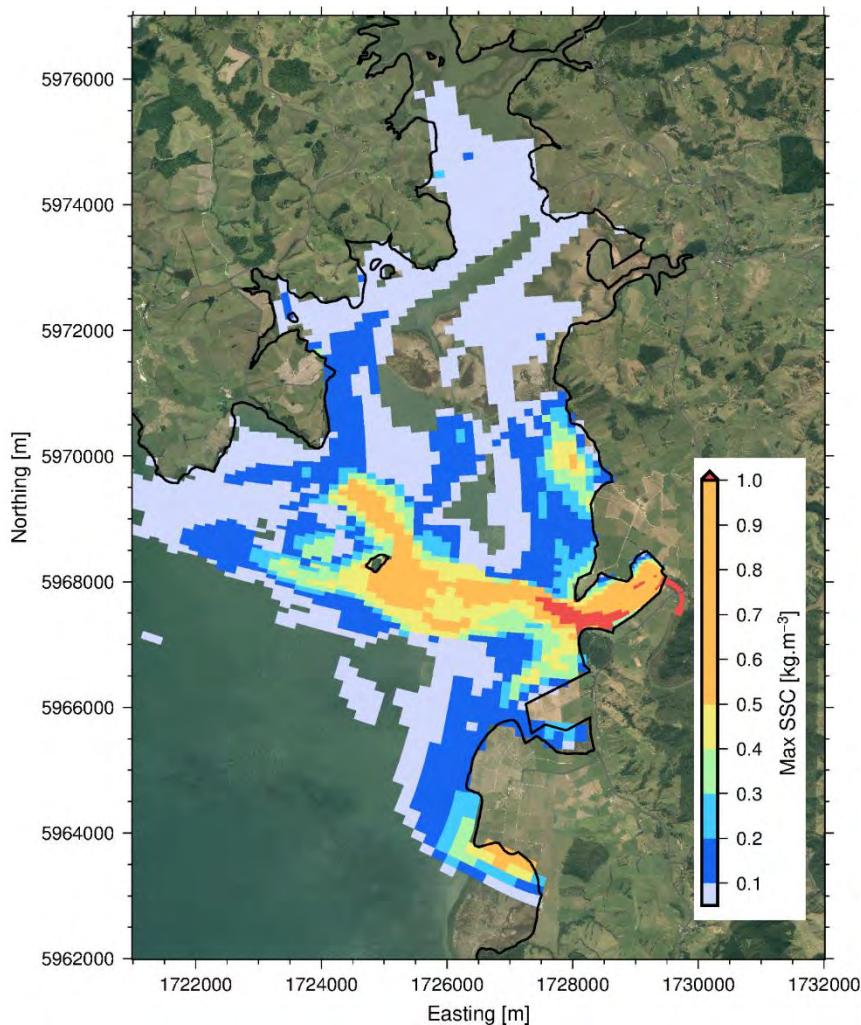
Figure 21: Maximum SSC for the base scenario of the 50-year ARI, calm wind event. Note: Sediment concentration below 0.05 \text{ kg/m}^3 are not shown here.
