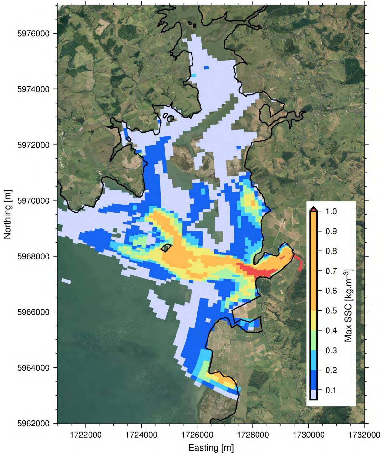
Figure 40: Maximum SSC for the base scenario of the 50-year ARI, calm wind event. Note: Sediment concentration below 0.005 \text{ kg}/\text{m}^3 are not shown here.
