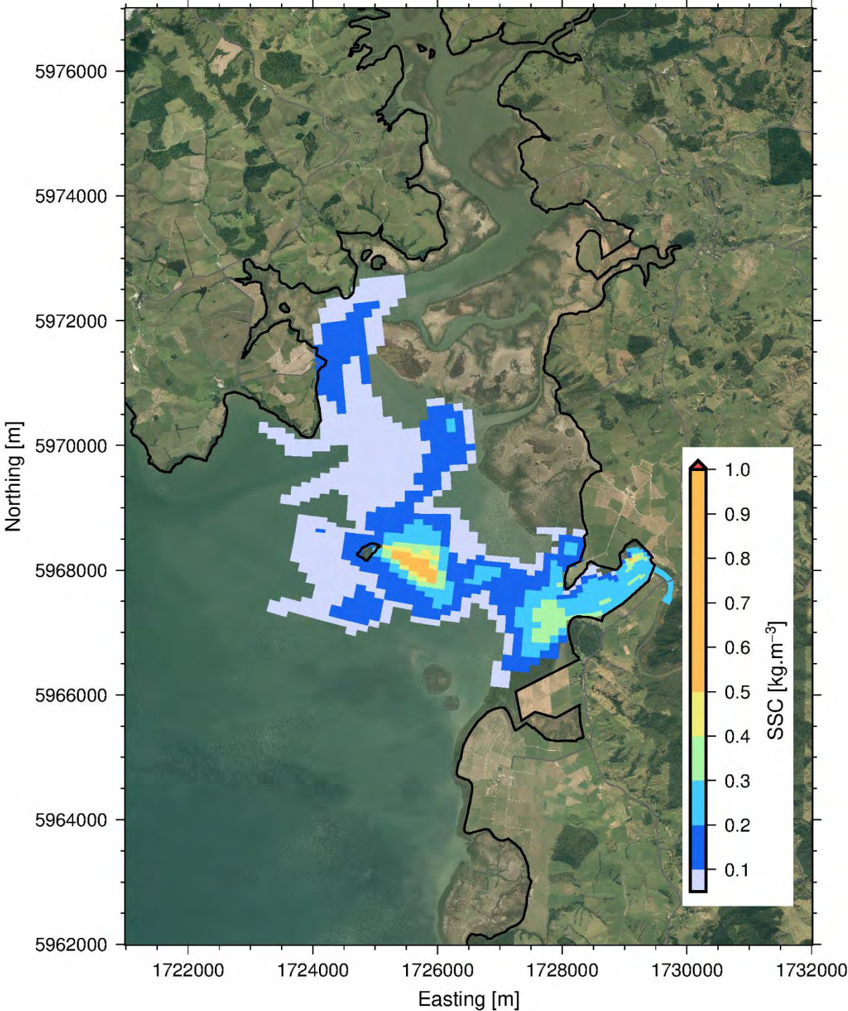
Figure 49: Suspended sediment concentration 1 day after the start of the event for the baseline 50-year ARI, calm wind event. Note the start of the event is when the suspended sediment concentration exceeds 0.01 kg/m 3 in the model input.
