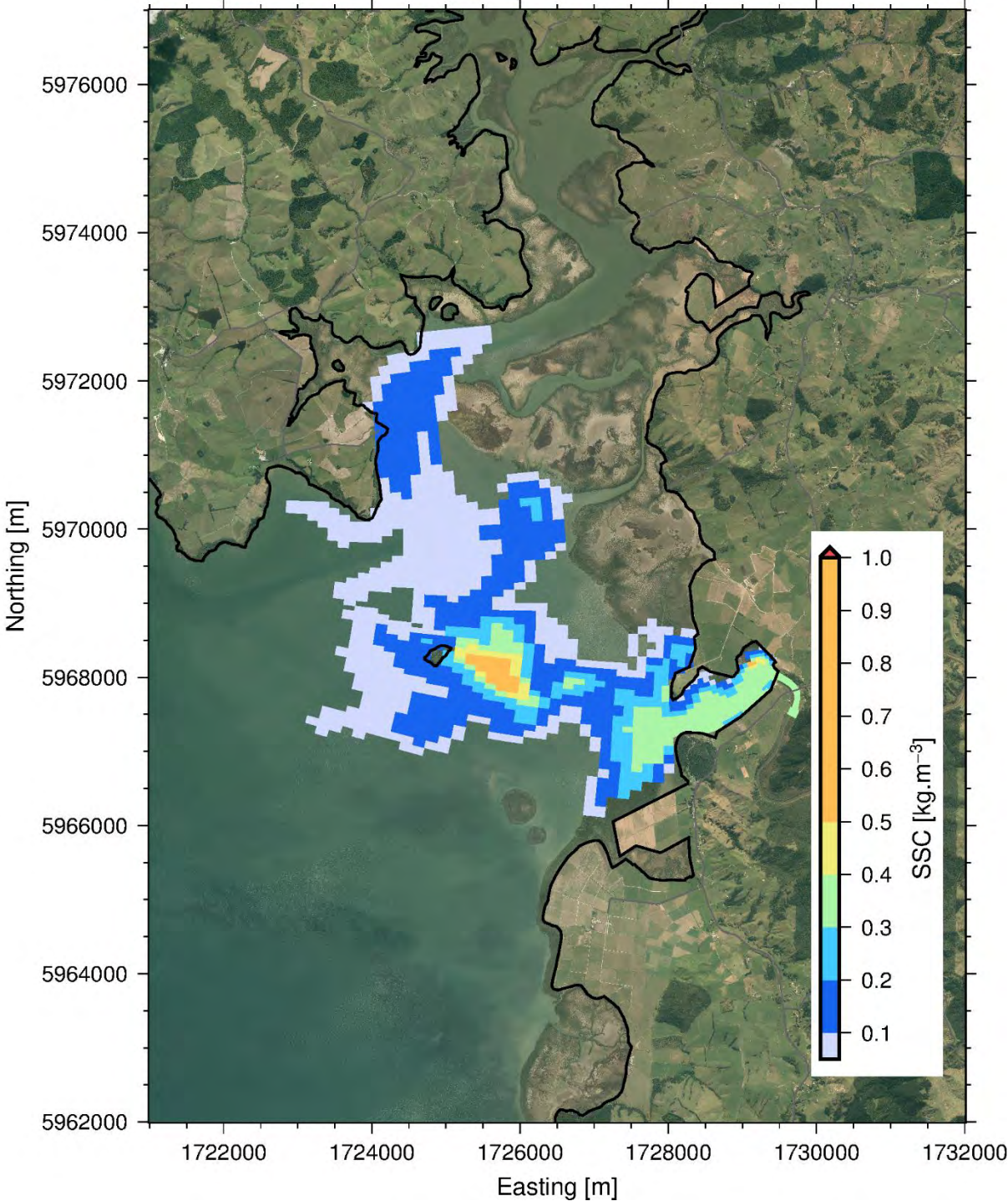
Figure 85: Suspended sediment concentration 1 day after the start of the event for the construction 50-year ARI, calm wind event. Note the start of the event is when the suspended sediment concentration exceeds 0.01 kg/m 3 in the model input.
