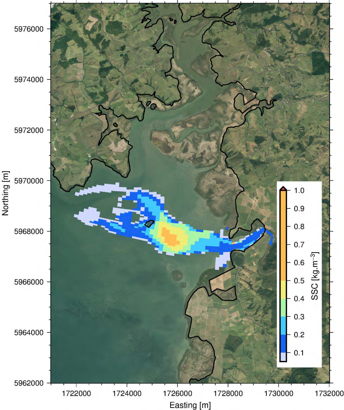
Figure 82: Suspended sediment concentration 3 days after the start of the event for the construction 10-year ARI, calm wind event. Note the start of the event is when the suspended sediment concentration exceeds 0.01 \text{ kg}/\text{m}^3 in the model input.
