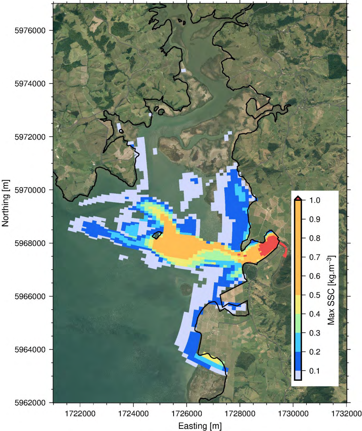
Figure 73: Maximum SSC for the construction scenario of the 10-year ARI, calm wind event. Note: Suspended sediment concentration below 0.005 \text{ kg}/\text{m}^3 are not shown here.
