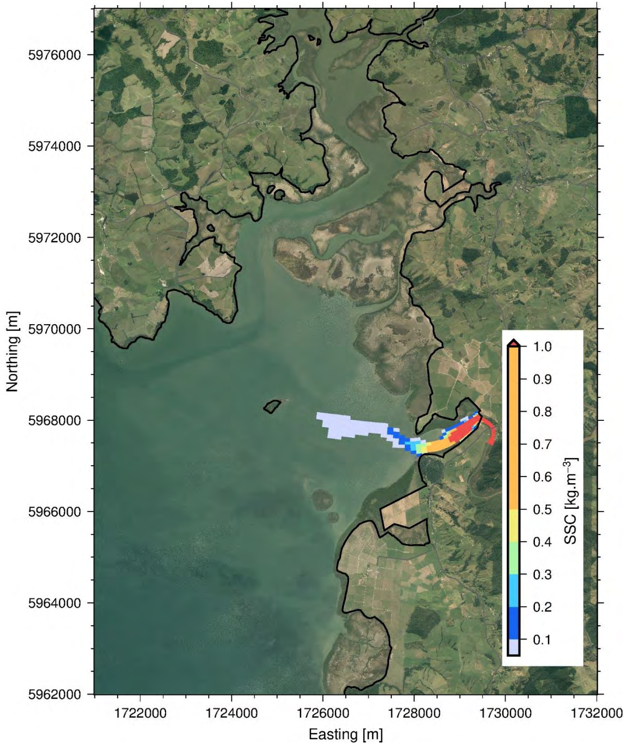
Figure 79: Suspended sediment concentration 1 day after the start of the event for the construction 10-year ARI, calm wind event. Note the start of the event is when the suspended sediment concentration exceeds 0.01 \text{ kg}/\text{m}^3 in the model input.
