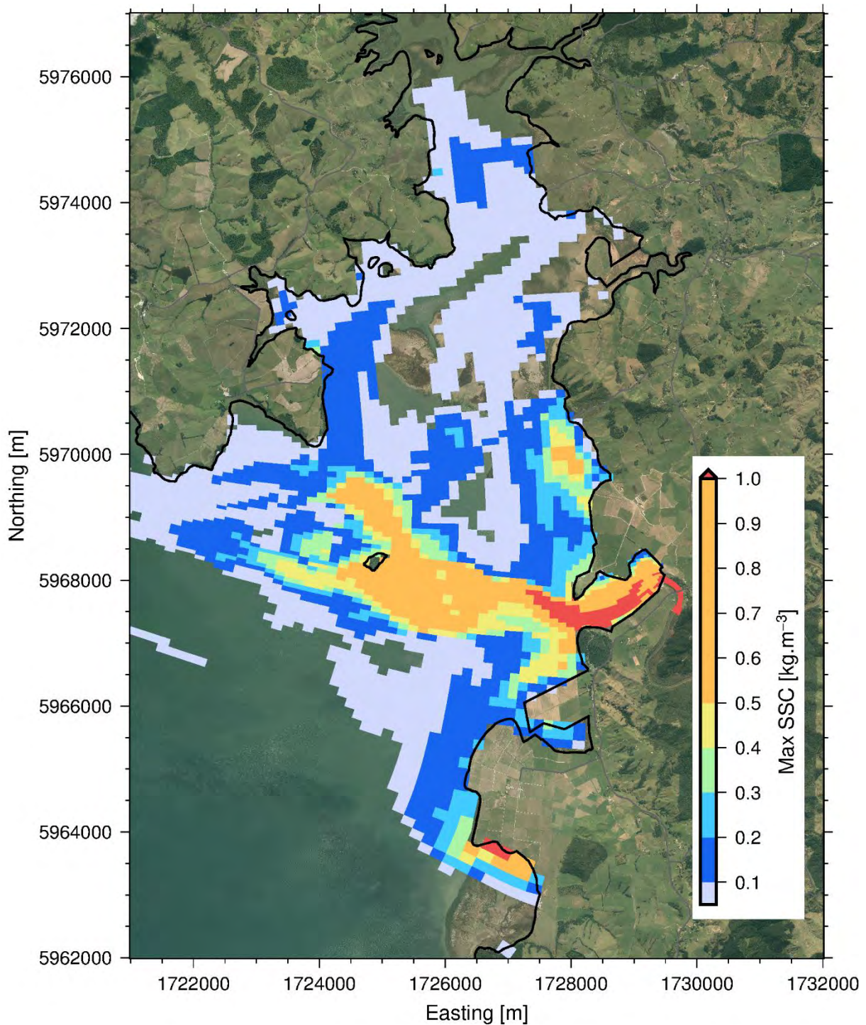
Figure 76: Maximum SSC for the construction scenario of the 50-year ARI, calm wind event. Note: Suspended sediment concentration below 0.005 \text{ kg}/\text{m}^3 are not shown here.
