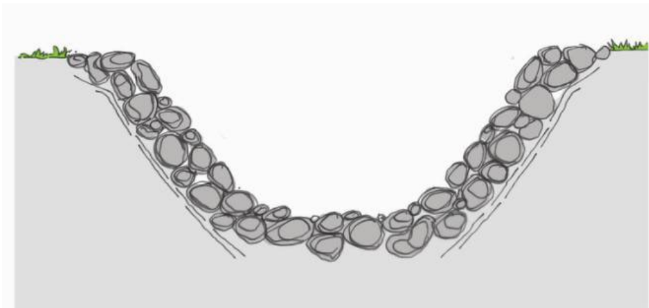
Rock-Lined Flow Channel for High Flow and/or Steep Gradients
