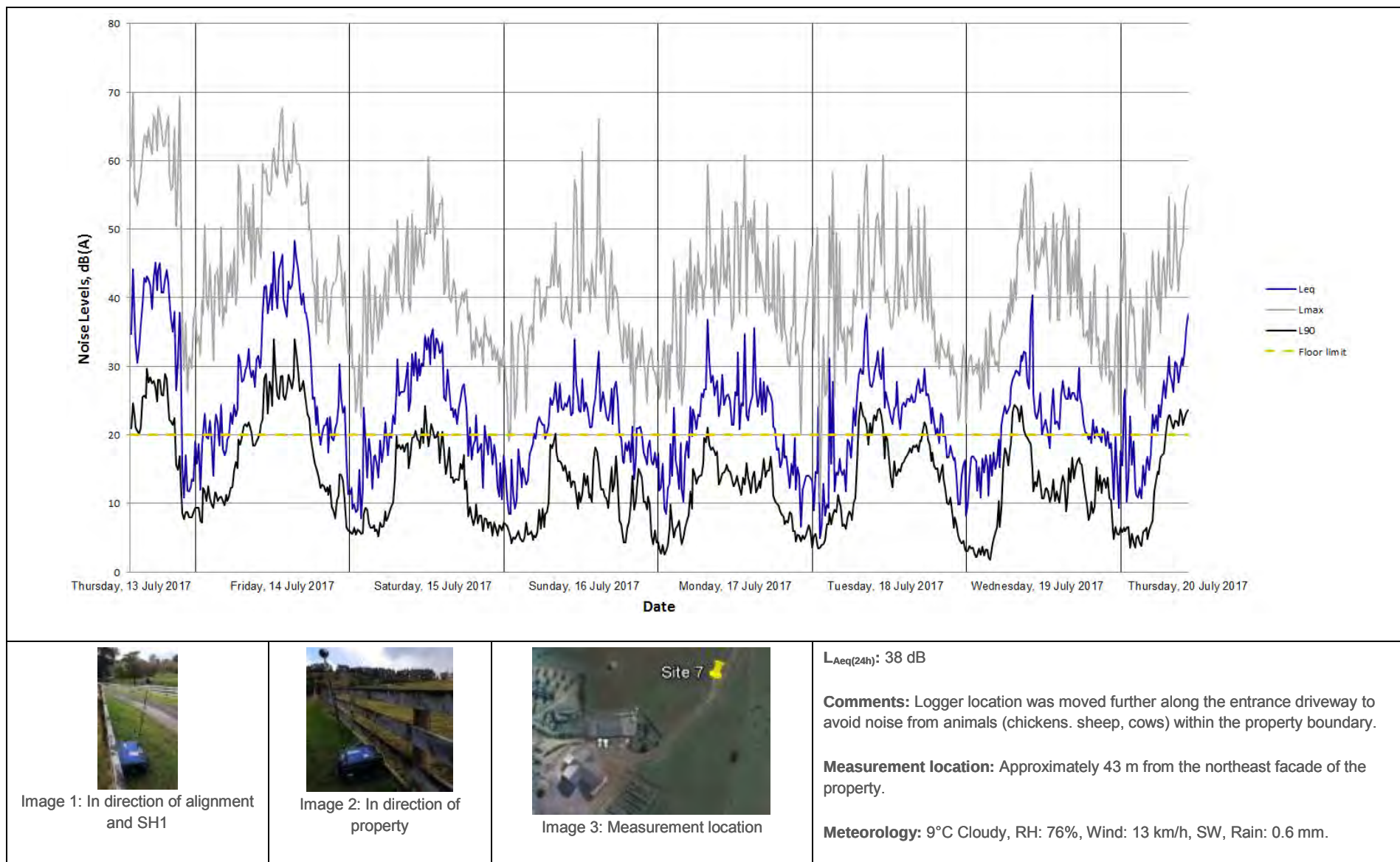
Figure 23 – Noise monitoring results at 39 Phillips Road
