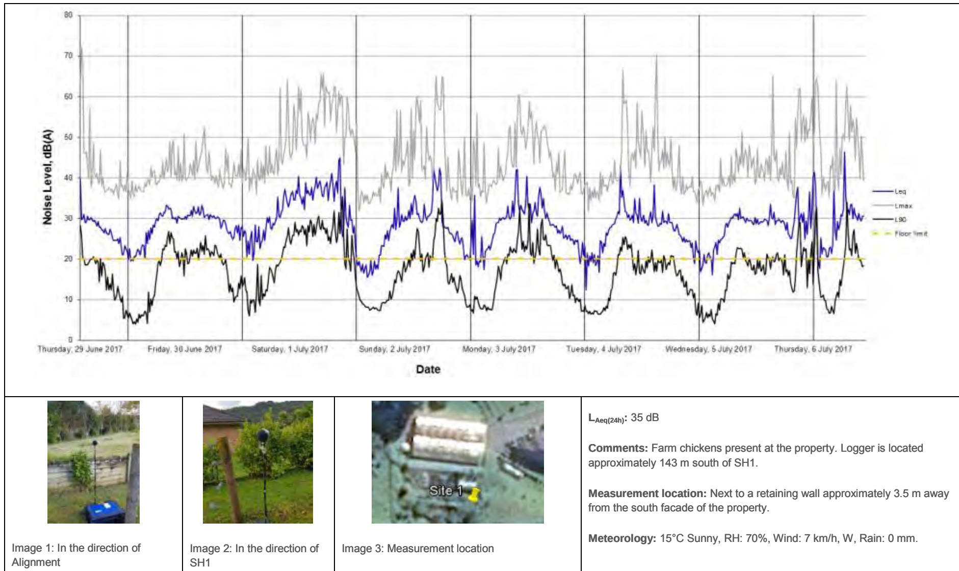
Figure 17 – Noise monitoring results at 761A SH1, Dome Forest
