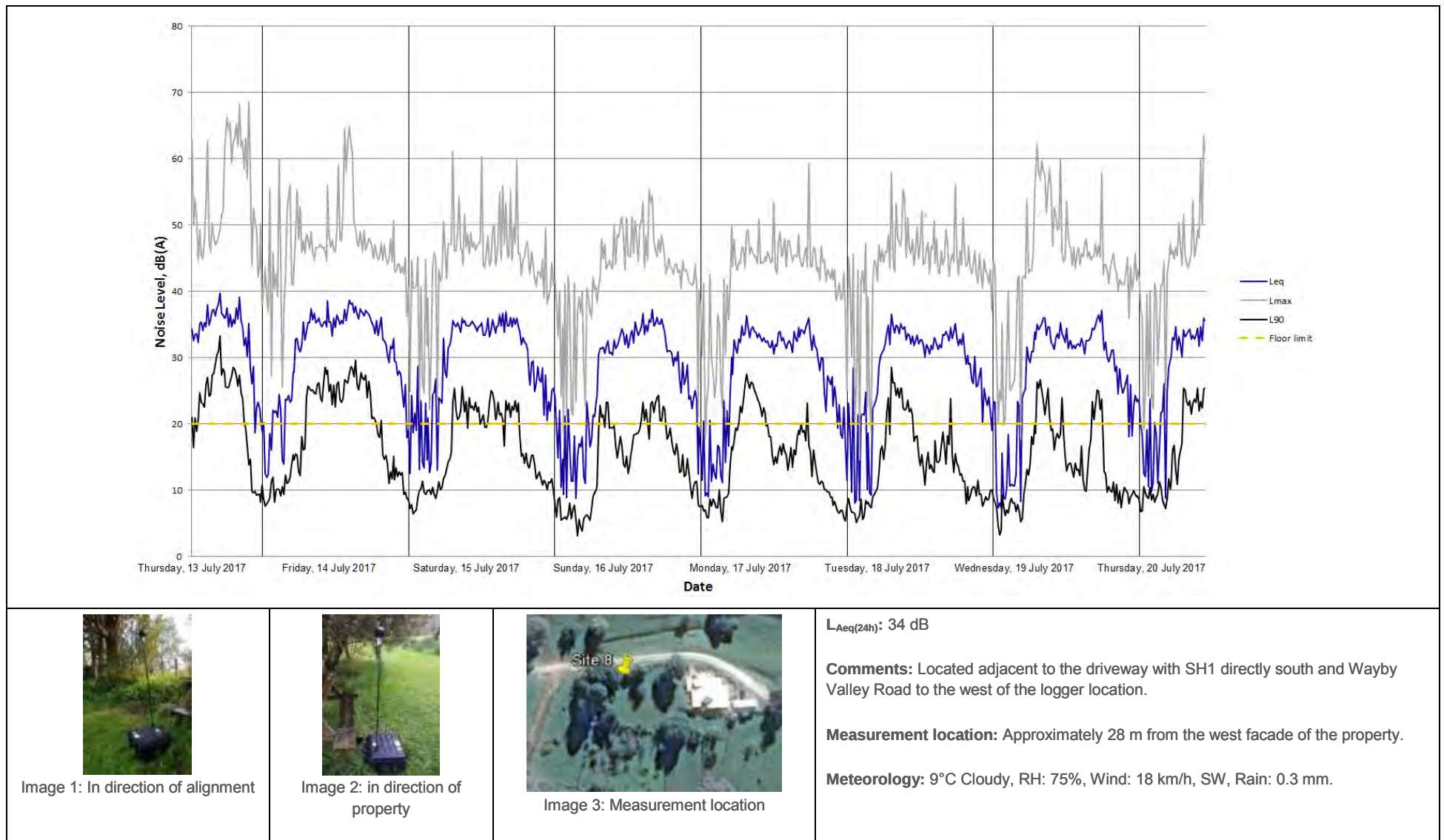
Figure 24 – Noise monitoring results at 294 Wayby Valley Road
