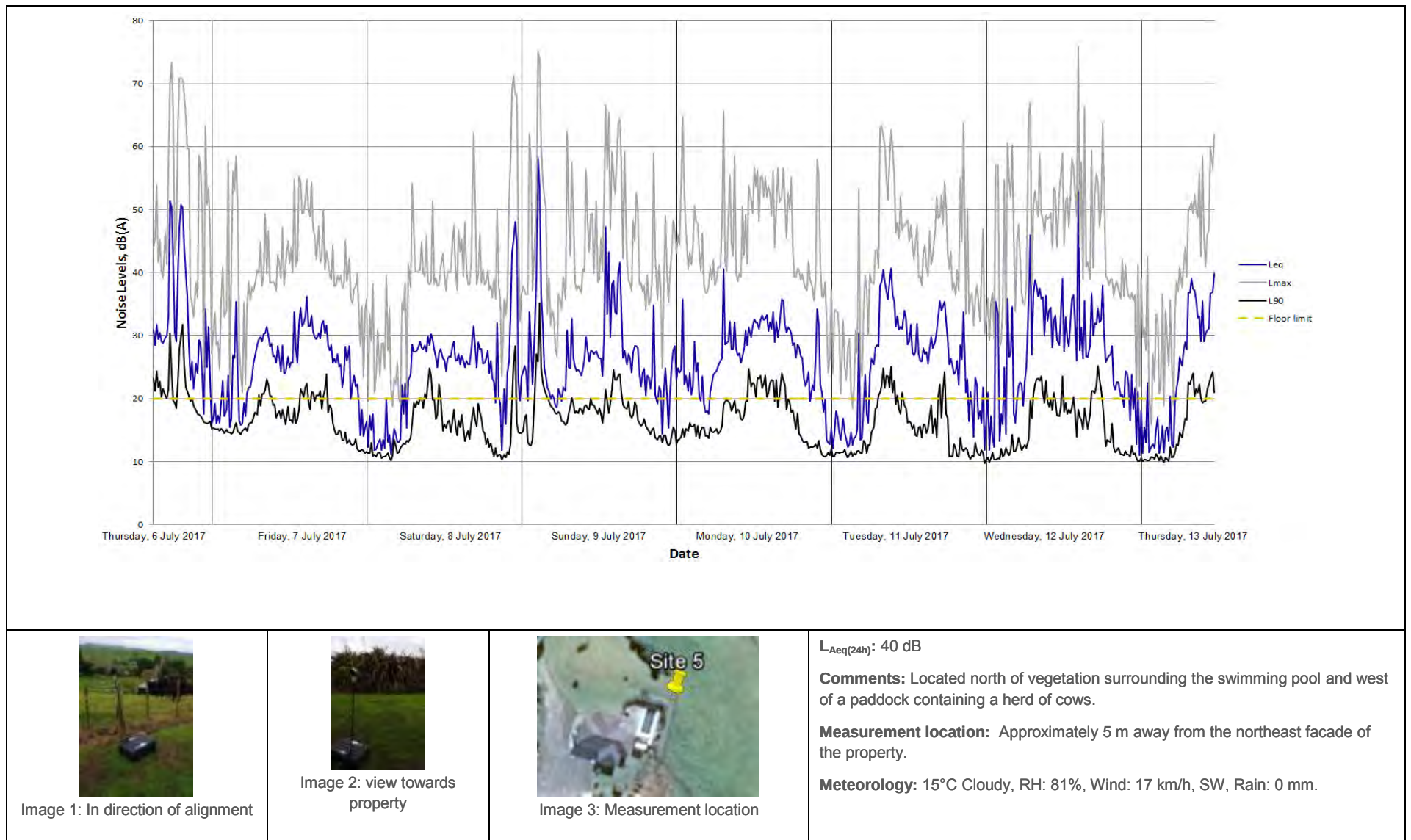
Figure 21 – Noise monitoring results at 40 Borrows Road
