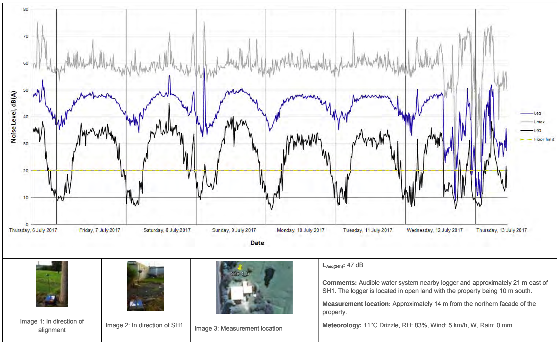
Figure 20 – Noise monitoring results at 490 SH1, Wellsford
