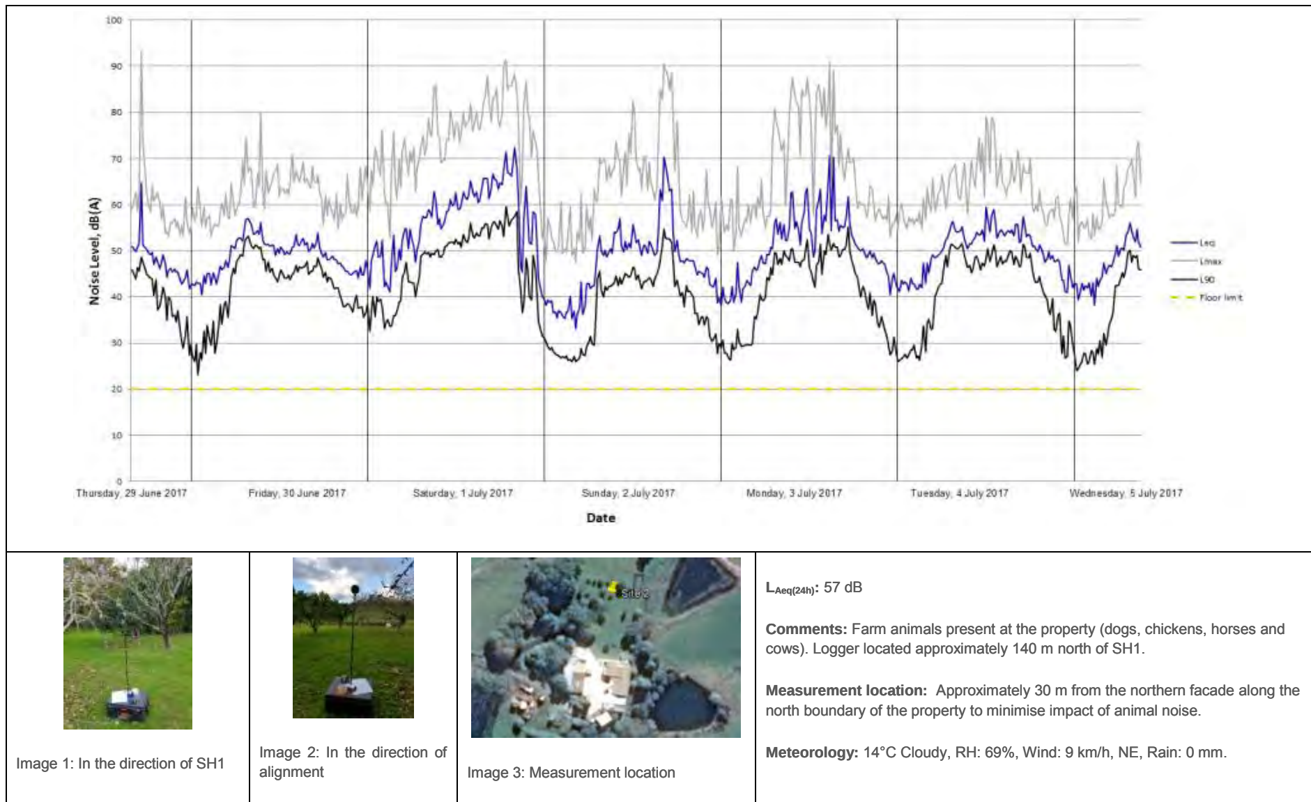
Figure 18 – Noise monitoring results at 1472 SH1, Wellsford
