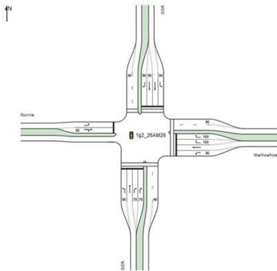
Figure 3-1: 2026 Signalised Intersection Layout
