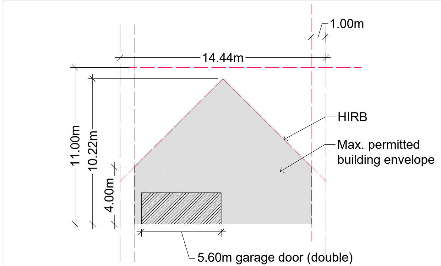
Example 1 - Operative Precinct Permitted Standards Max Building Bulk - 14.44m site width
