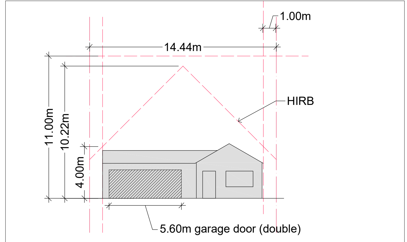
Example 2 - Example 1 but with single level
