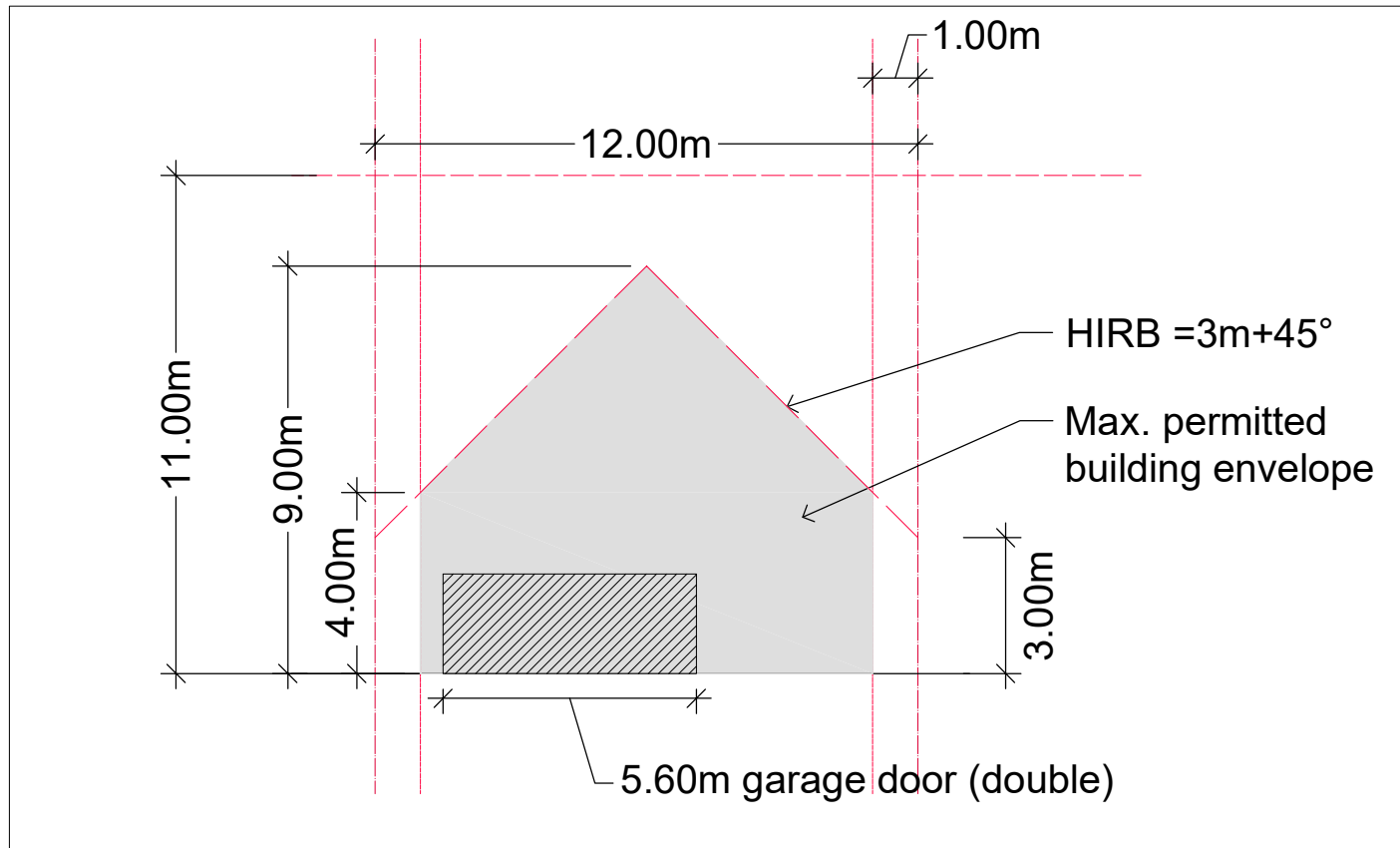
Example 3 - MHU Zone Permitted Standards - Max Building Bulk - 12m site
