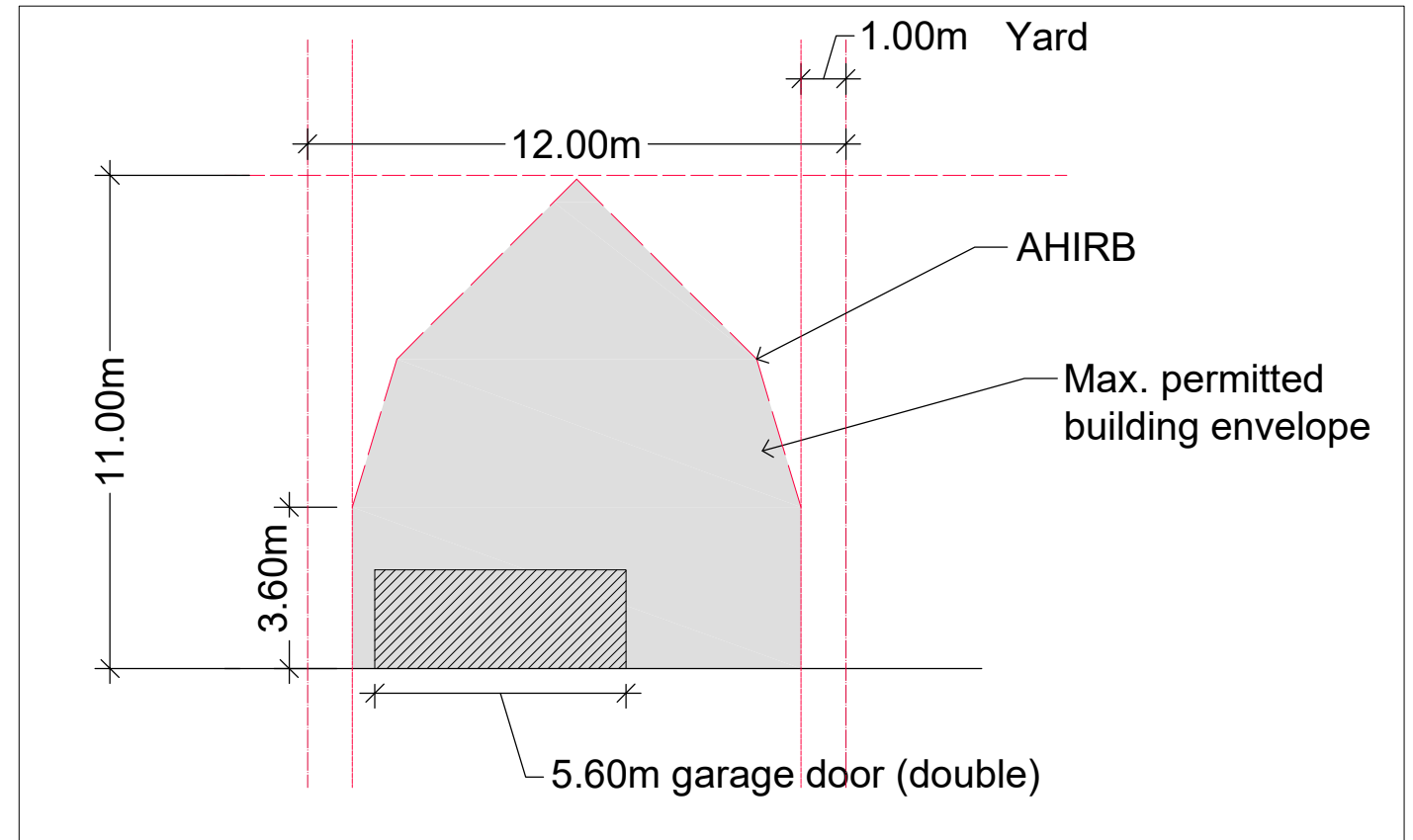
Example 4 - Proposed AHIRB Standards 12m site
