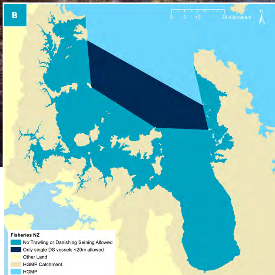
Figure 23: Difference between: a) the restrictions prescribed in fisheries regulations for Danish seining, and b) the restrictions applied by Fisheries NZ.
