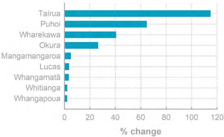
Figure 53: Percentage change in mangrove cover from 1993–2000 to 2012–2017. Data excludes the large-scale clearances that have since occurred in Whangamatā and Tairua. Most of the data was mapped from aerial photographs. Some GIS layers were provided by WRC. Aerials for the start period for Okura, Lucas, Mangamangaroa and Whitianga were not available and this data was taken from the literature 102,109 . The 2000 aerial photograph for Whangapoua was provided by NIWA with permission from Ernslaw One.
