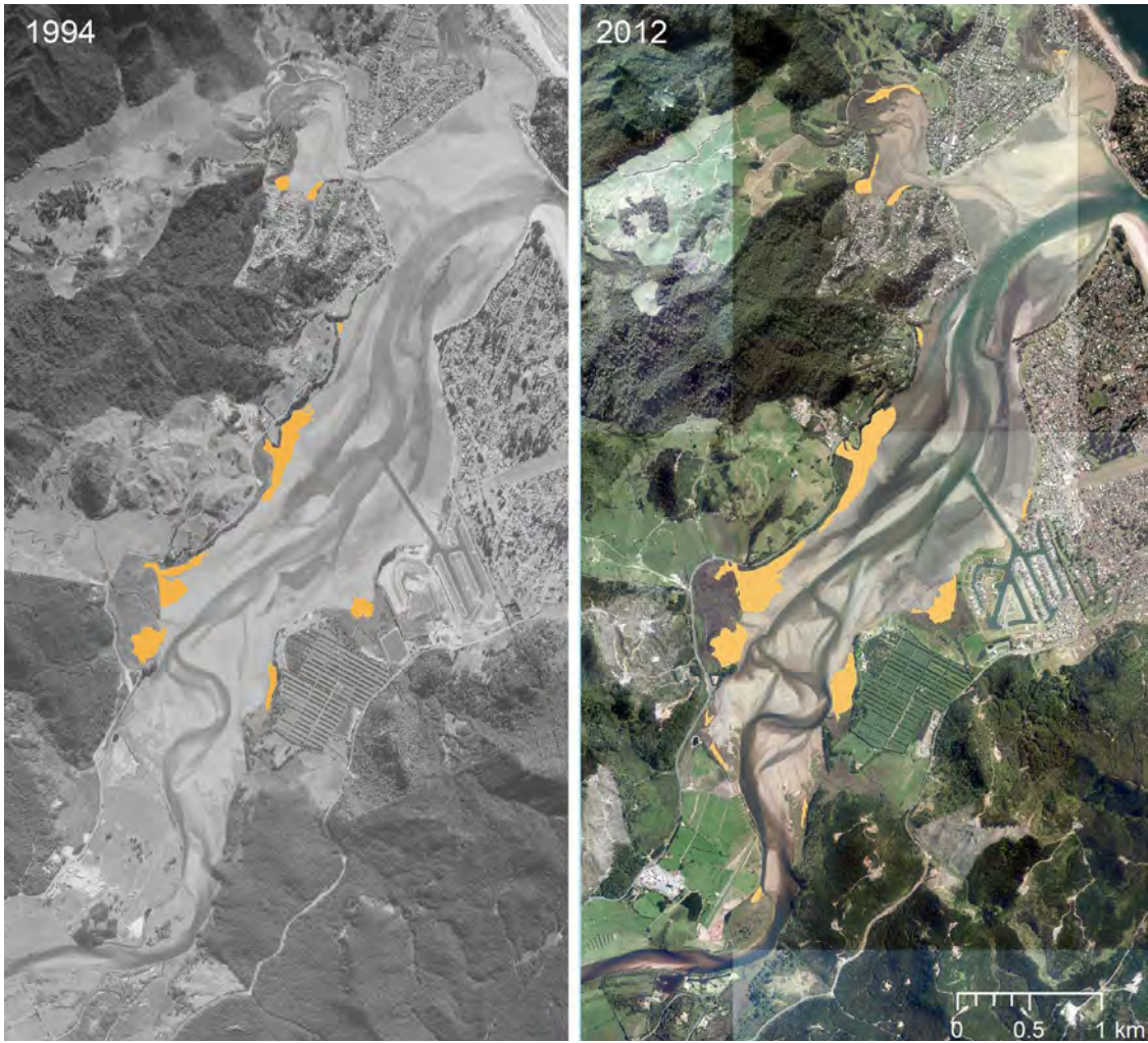
Figure 54: Changes in the mangrove cover (orange areas) in Tairua Estuary between 1994 and 2012.
