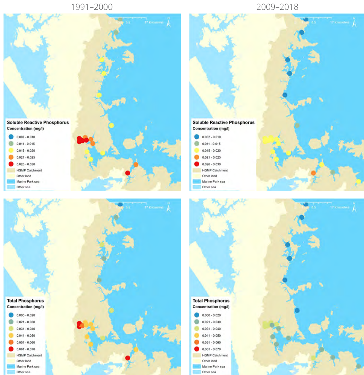
Figure 38: Median soluble reactive phosphorus (top) and total phosphorus (bottom) concentrations at monitored coastal sites between 1991-00 and 2009-18.
