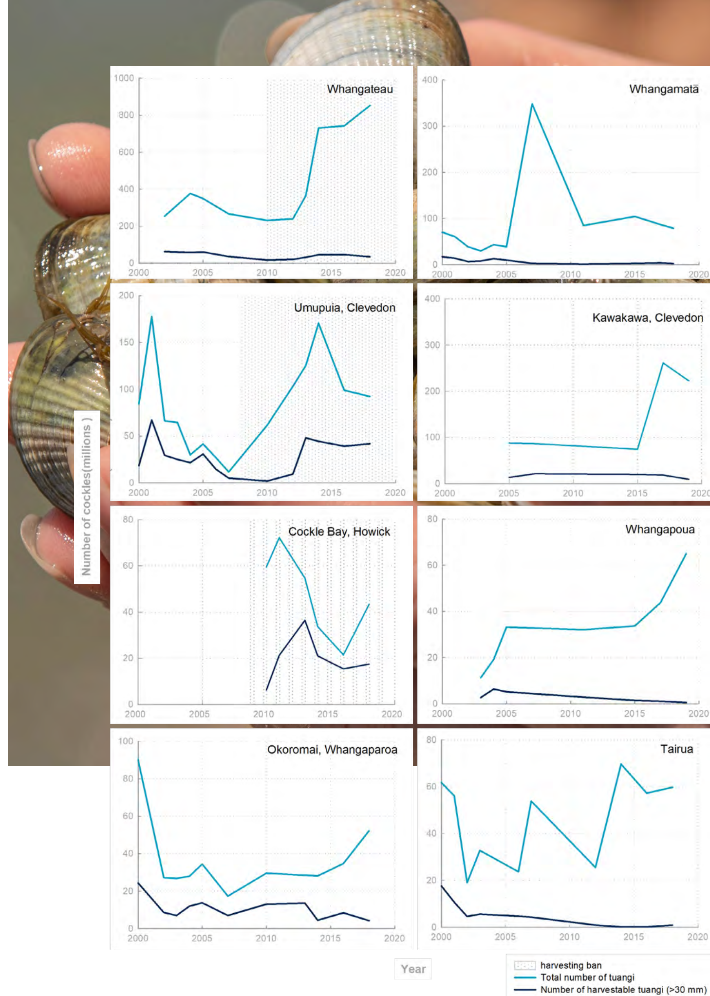
Figure 19: Estimated total number of tuangi and number of harvestable tuangi at Marine Park sites that have been regularly monitored by MPI since 2000.
