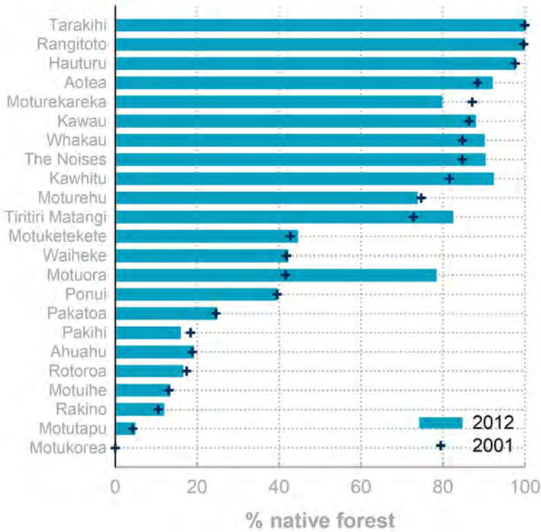
Figure 64: Change in the percentage of island covered by native forests between 2001 and 2012. Data from LCDB 2 and LCDB 4.1.
