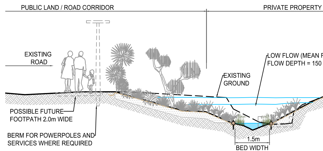
SECTION B - OPEN CHANNEL DETAIL - TUI ST TO NIKAU RD - CHAINAGE 100 (P2)
