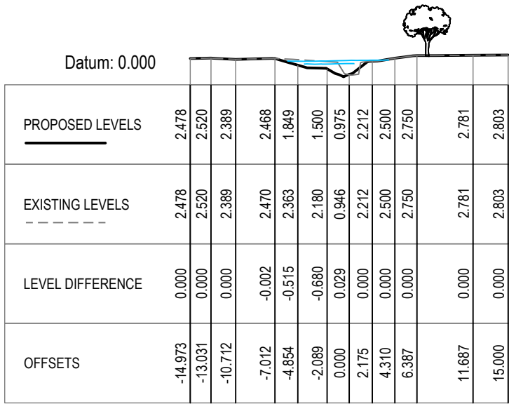
CHAINAGE 120.000
