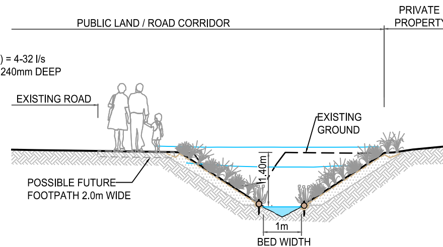
SECTION D - OPEN CHANNEL DETAIL - TUI ST TO NIKAU RD - CHAINAGE 280
