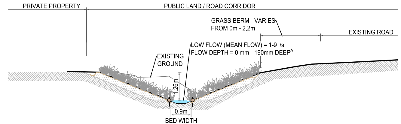
SECTION F - OPEN CHANNEL DETAIL - MOA AVE NORTH - CHAINAGE 20 (P6)
