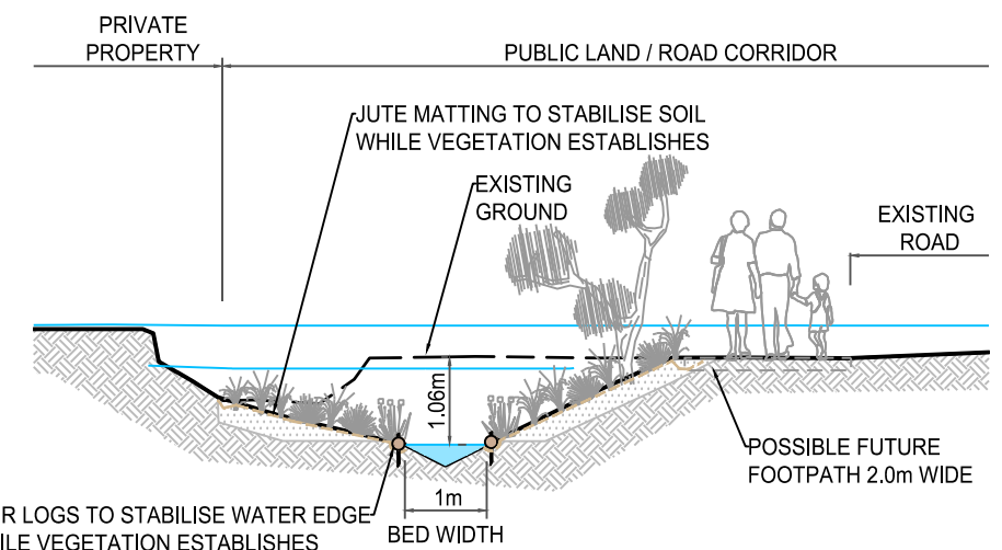
SECTION E - OPEN CHANNEL DETAIL - TUI ST TO NIKAU RD - CHAINAGE 340
