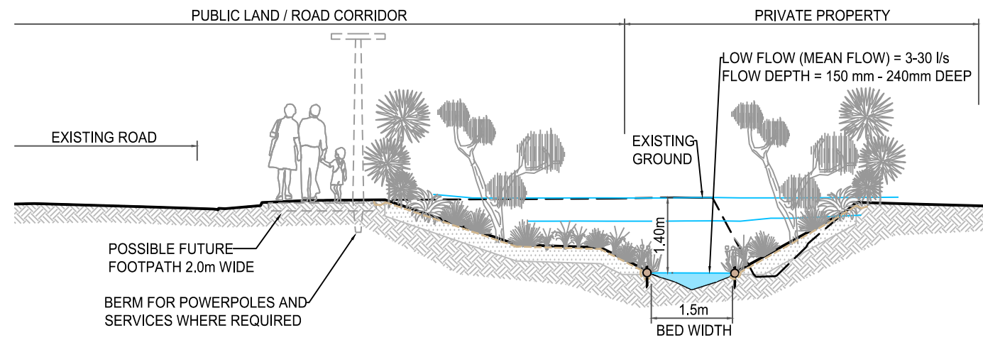
SECTION C - OPEN CHANNEL DETAIL - TUI ST TO NIKAU RD - CHAINAGE 200 (P3)
