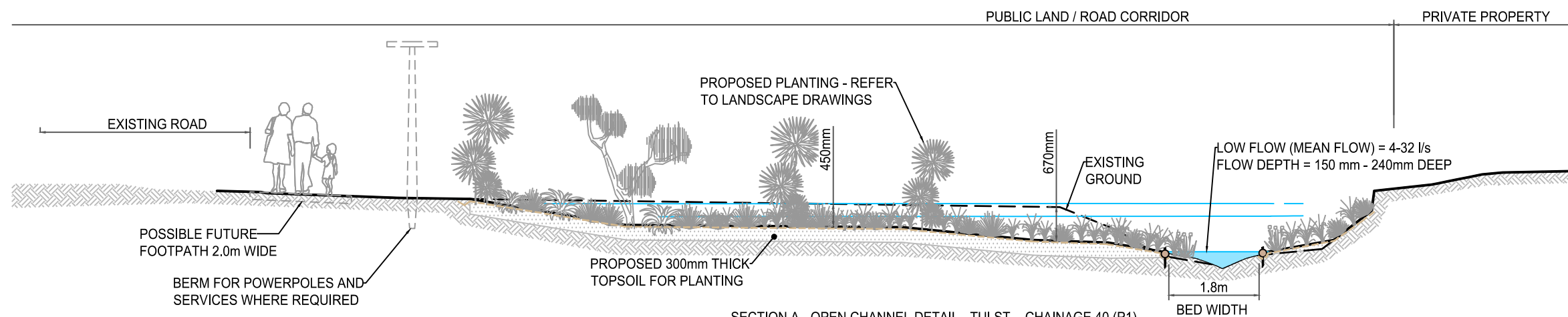
SECTION A - OPEN CHANNEL DETAIL - TUI ST - CHAINAGE 40 (P1)
