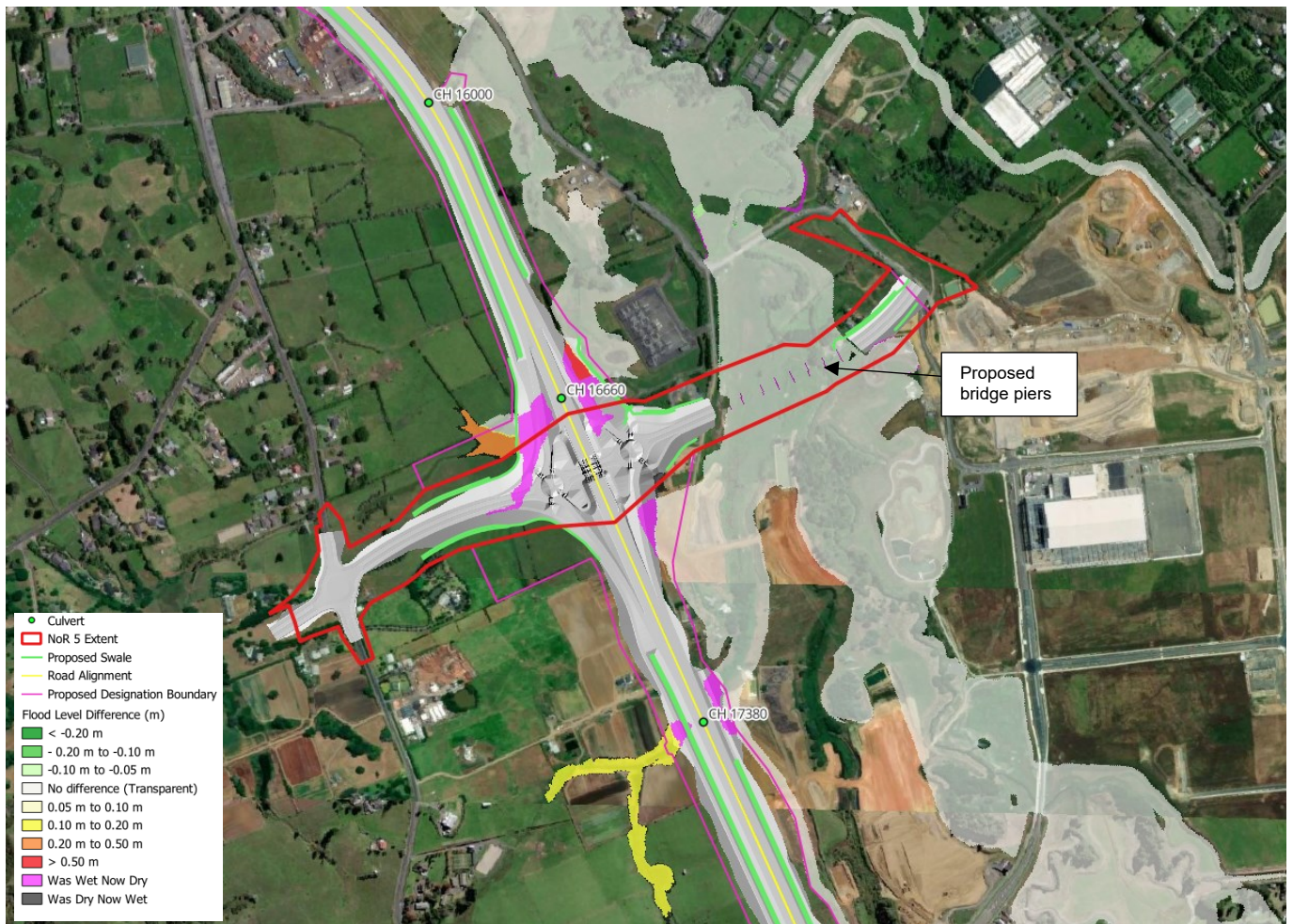
Figure 10-4 Flood impact (post-development vs pre-development) for the 1% AEP event with climate change – NoR 5
