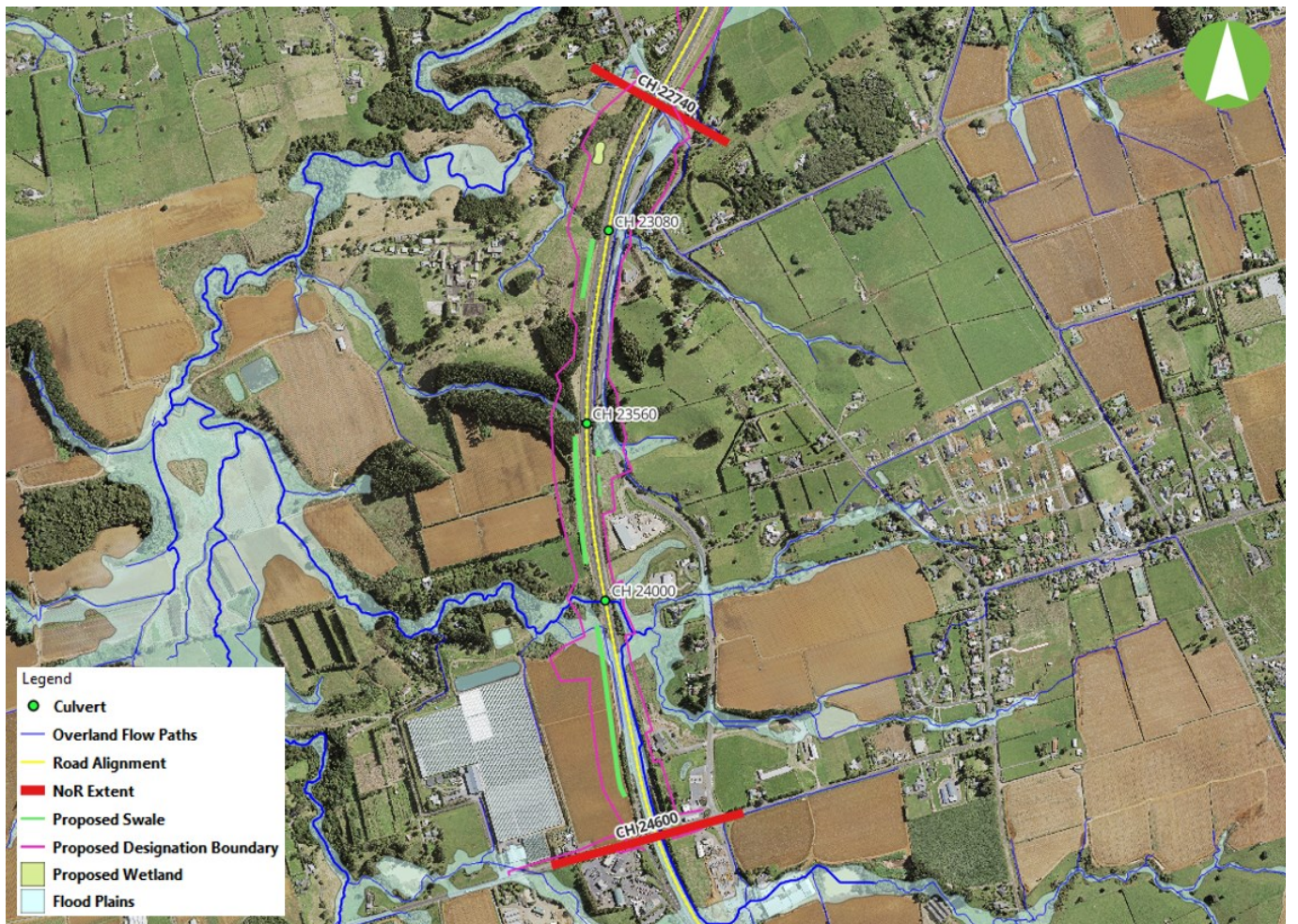
Figure 8-3 Proposed swale locations within NoR 3 project boundary
