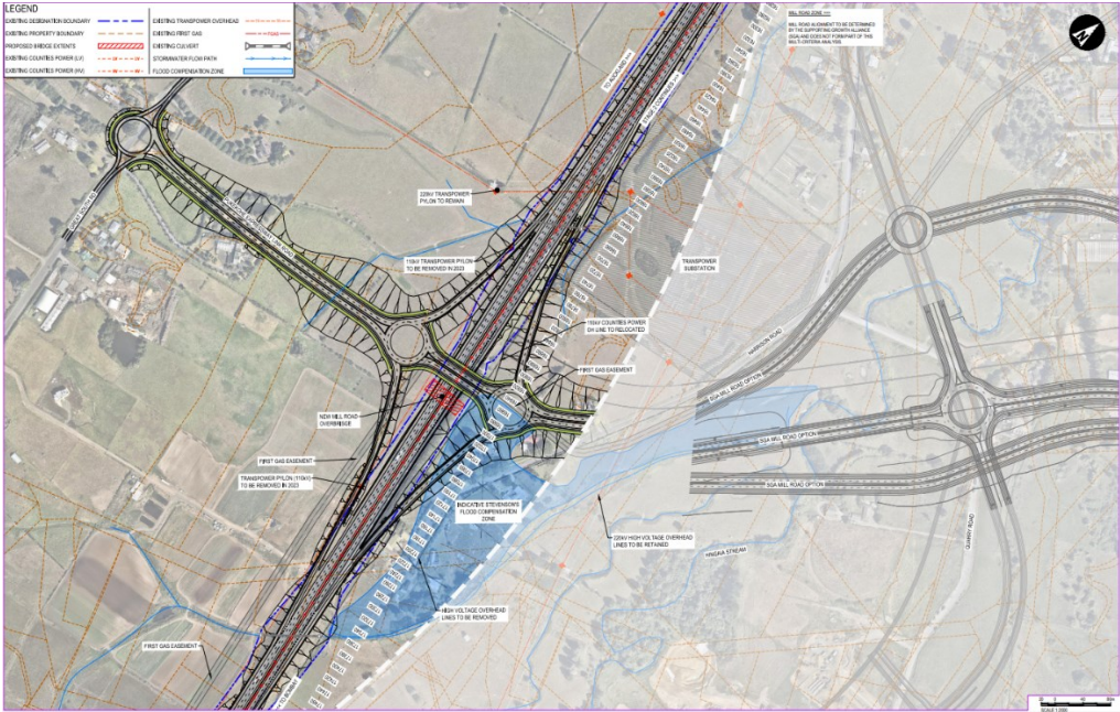
Figure 5-4 Drury South Interchange Option 1 (Option 2020-1)
