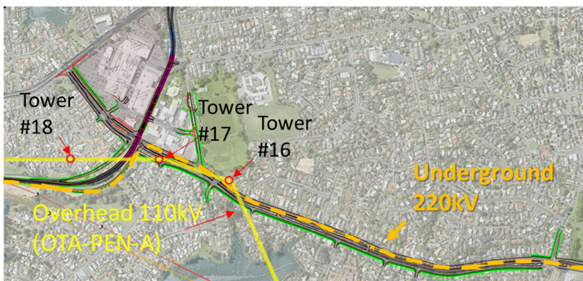
Figure 4 – High Voltage Transmission Plan
