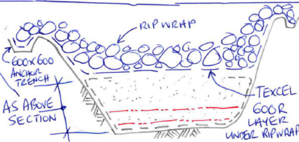
TYPICAL RIP WRAP CROSS SECTION
