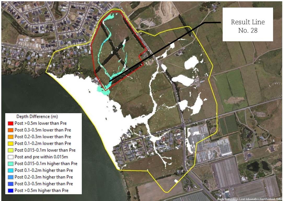
FIGURE 22: 1% AEP depth difference, ED + MPD minus ED flood model scenarios (1 m SLR).
