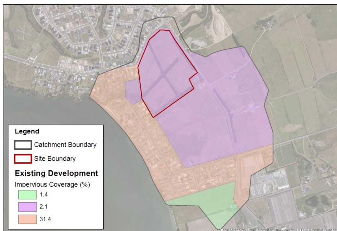
FIGURE 15: ED scenario model extent and imperviousness.
