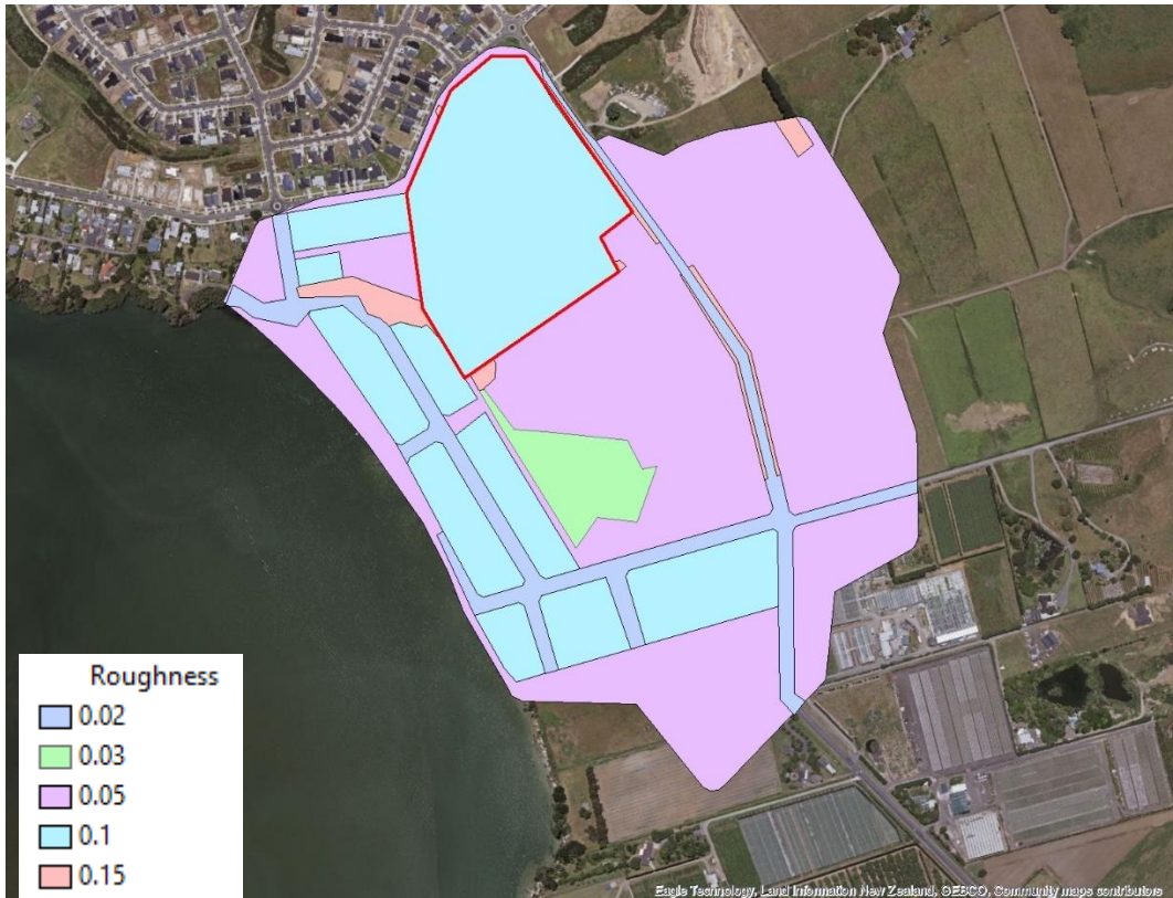
FIGURE 19: Hydraulic model MPD and MPD+ED scenario surface roughness values (Manning's n values).
