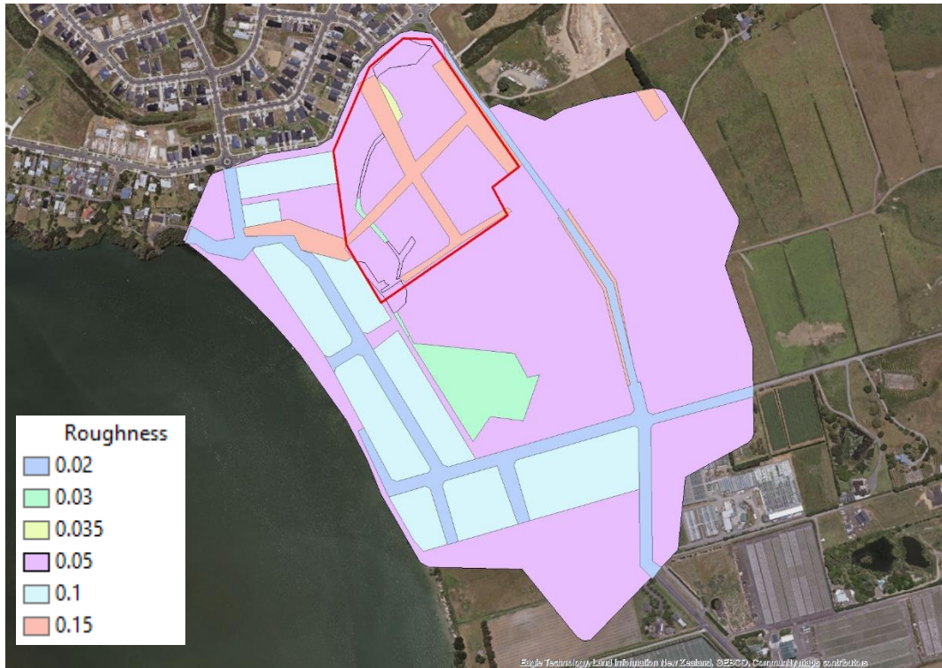
FIGURE 18: Hydraulic model ED scenario surface roughness values (Manning's n values).
