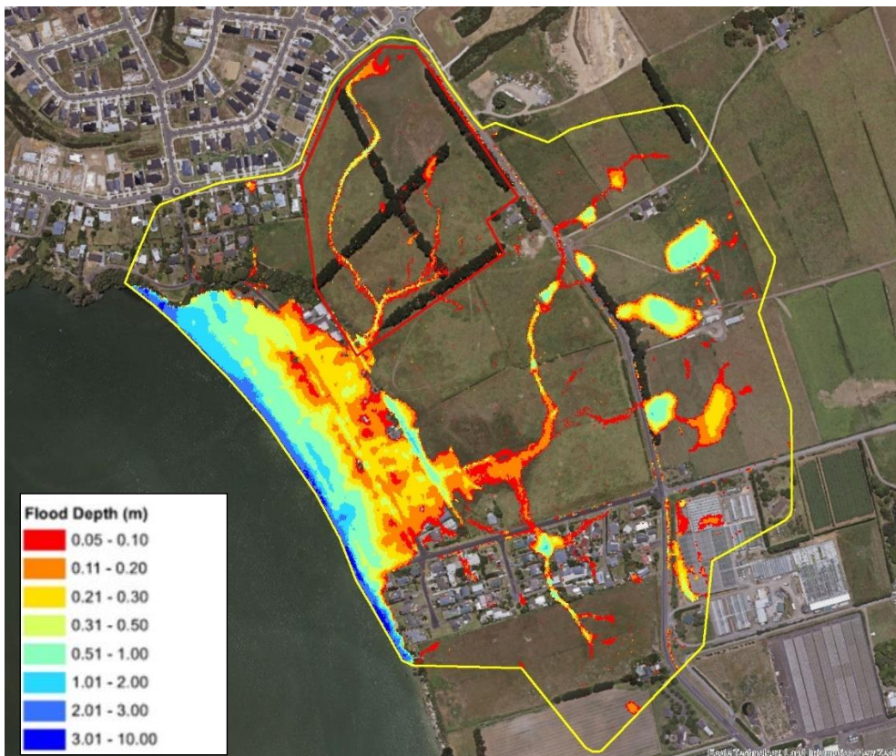
FIGURE 21: Existing Development scenario, 1% AEP hydraulic model results (1 m SLR).
