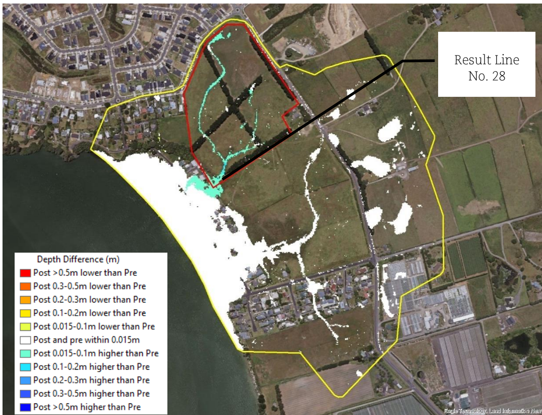
FIGURE 23: 10% AEP depth difference, ED + MPD minus ED flood model scenarios (1 m SLR).
