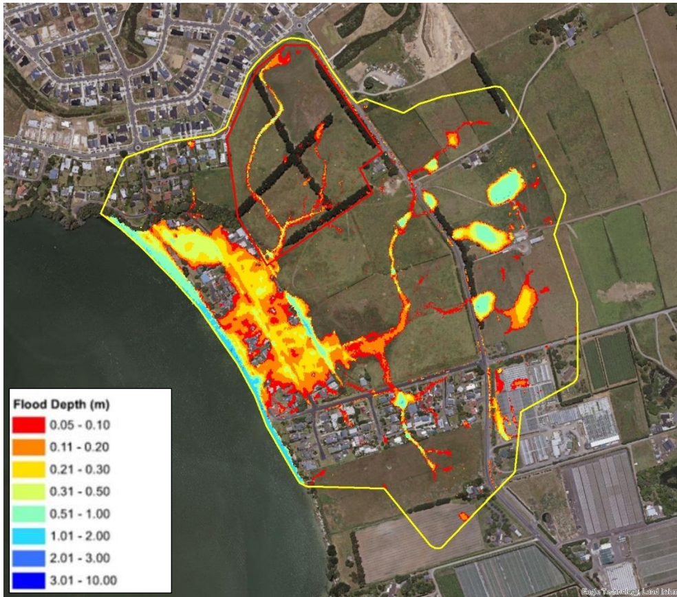
FIGURE 20: Existing Development scenario, 1% AEP hydraulic model results (no SLR).
