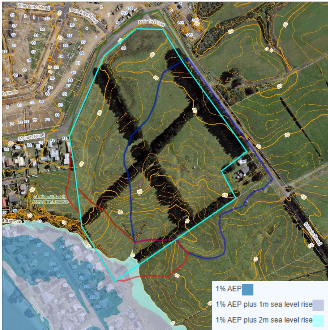
FIGURE 14: Coastal inundation extents (Auckland Council, 2022).
