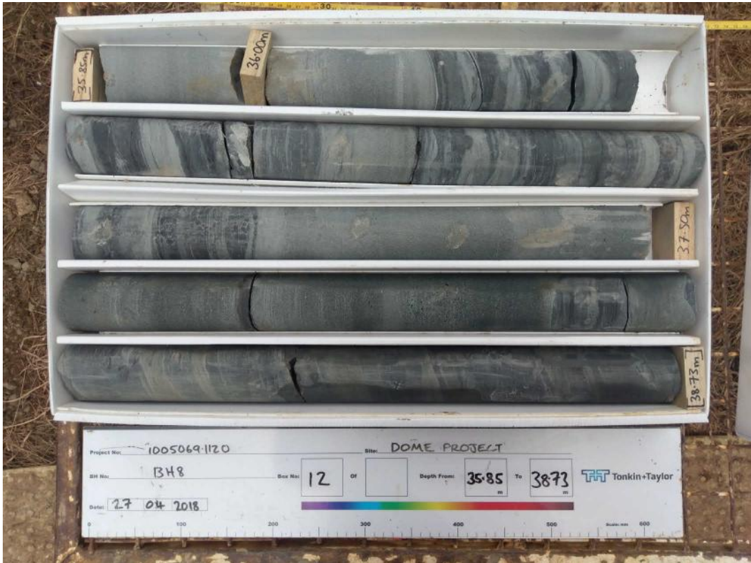
BOX 12 35.85-38.73m
