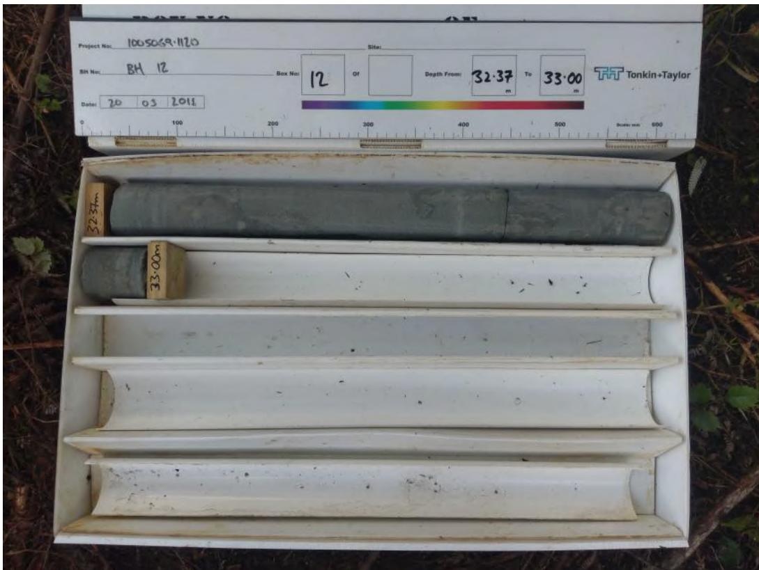
BOX 12 32.37-33.00m
