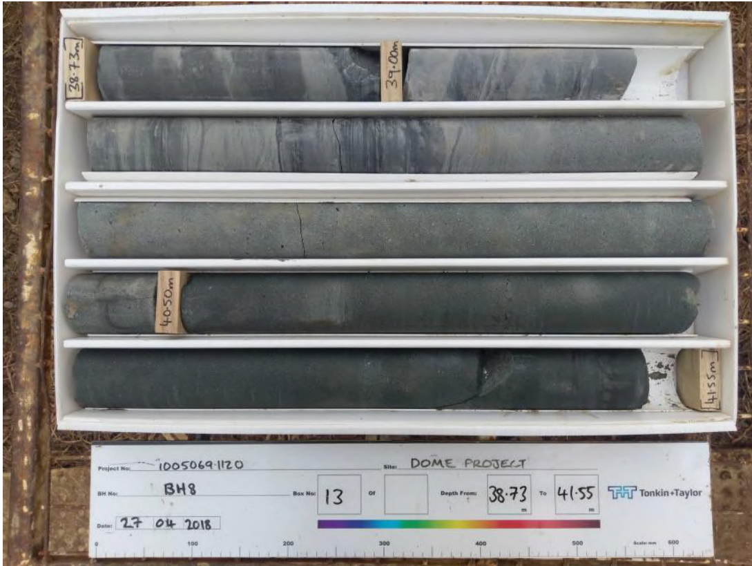
BOX 13 38.73-41.55m
