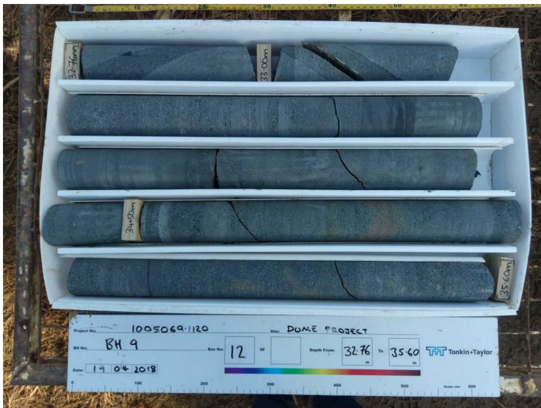
BOX 12 32.76-35.60m
