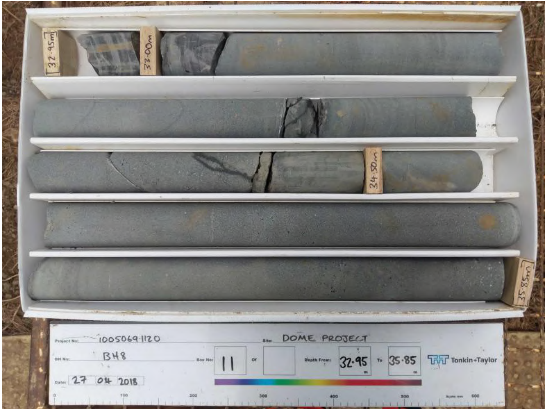
BOX 11 32.95-35.85m
