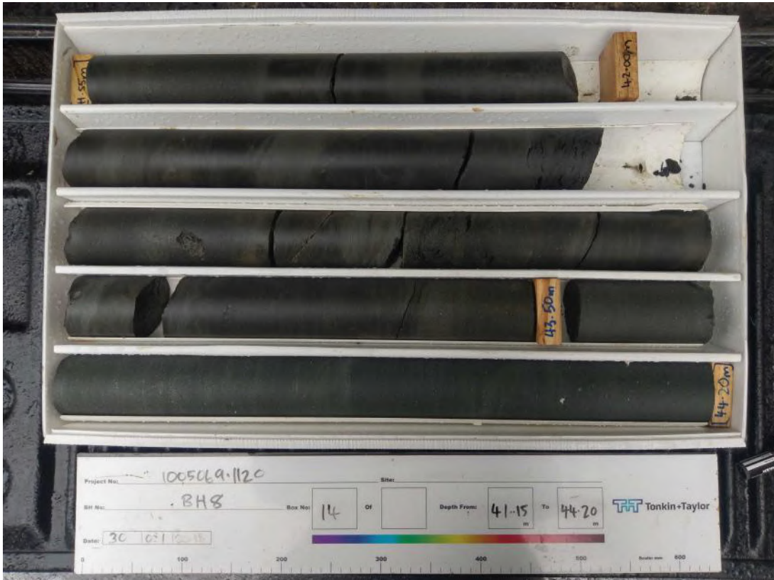
BOX 14 41.55-44.20m
