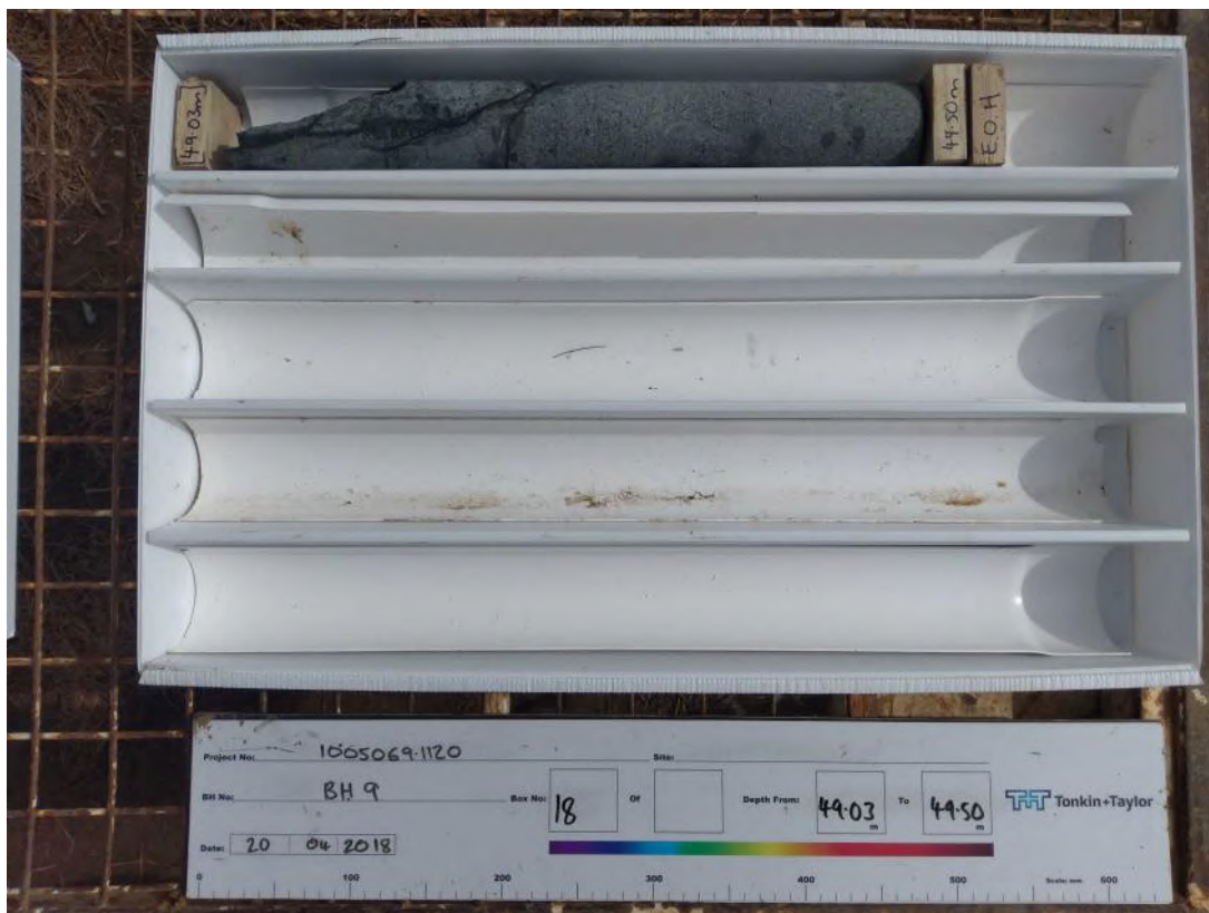
BOX 18 49.03-49.50m
