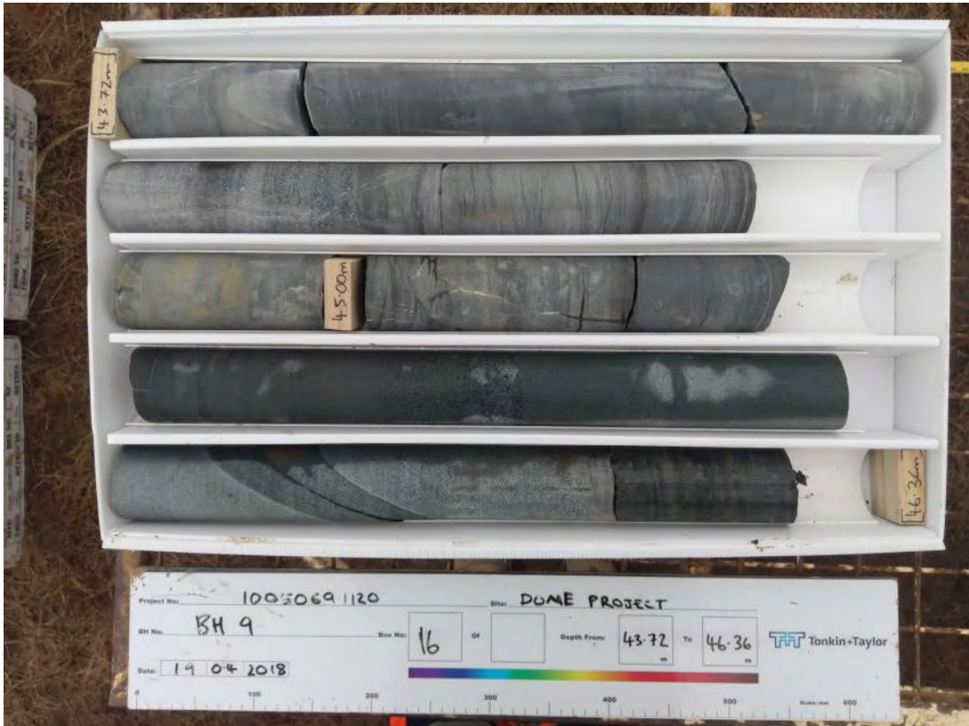
BOX 16 43.72-46.36m
