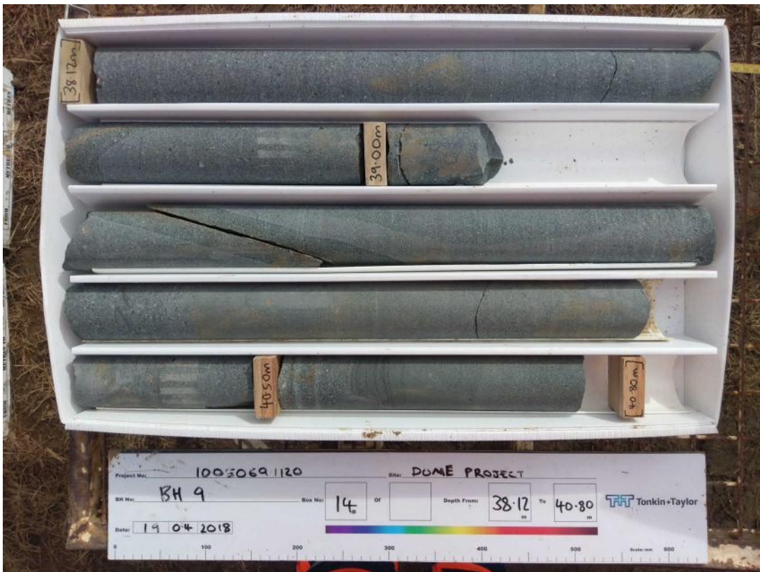
BOX 14 38.12-40.80m
