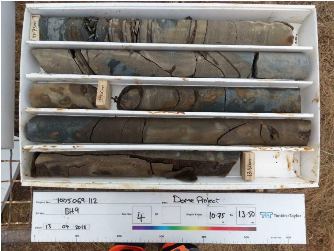
BOX 4 10.75-13.50m
