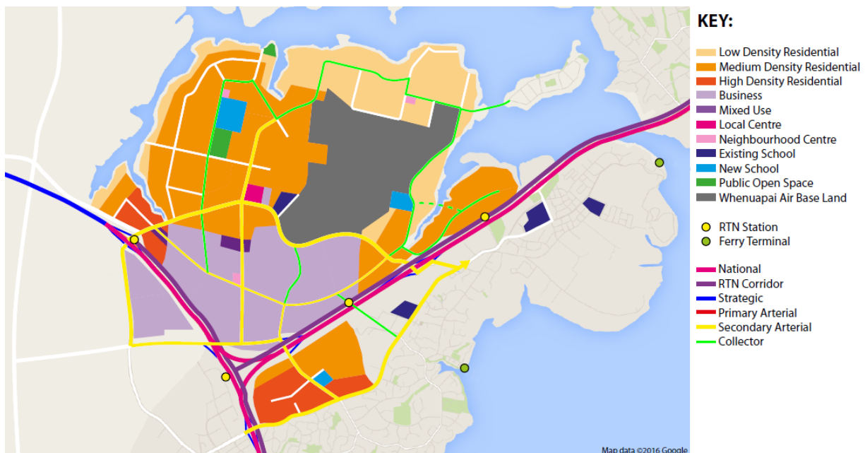
Figure 6: Assessed Whenuapai Structure Plan and Transport Network
