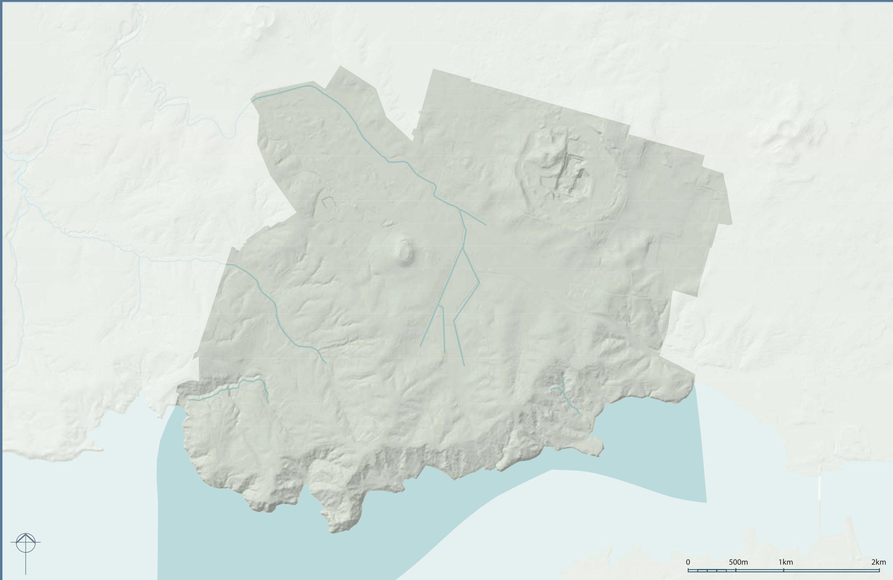
Map A1.1 - GEOMORPHOLOGY Terrain
