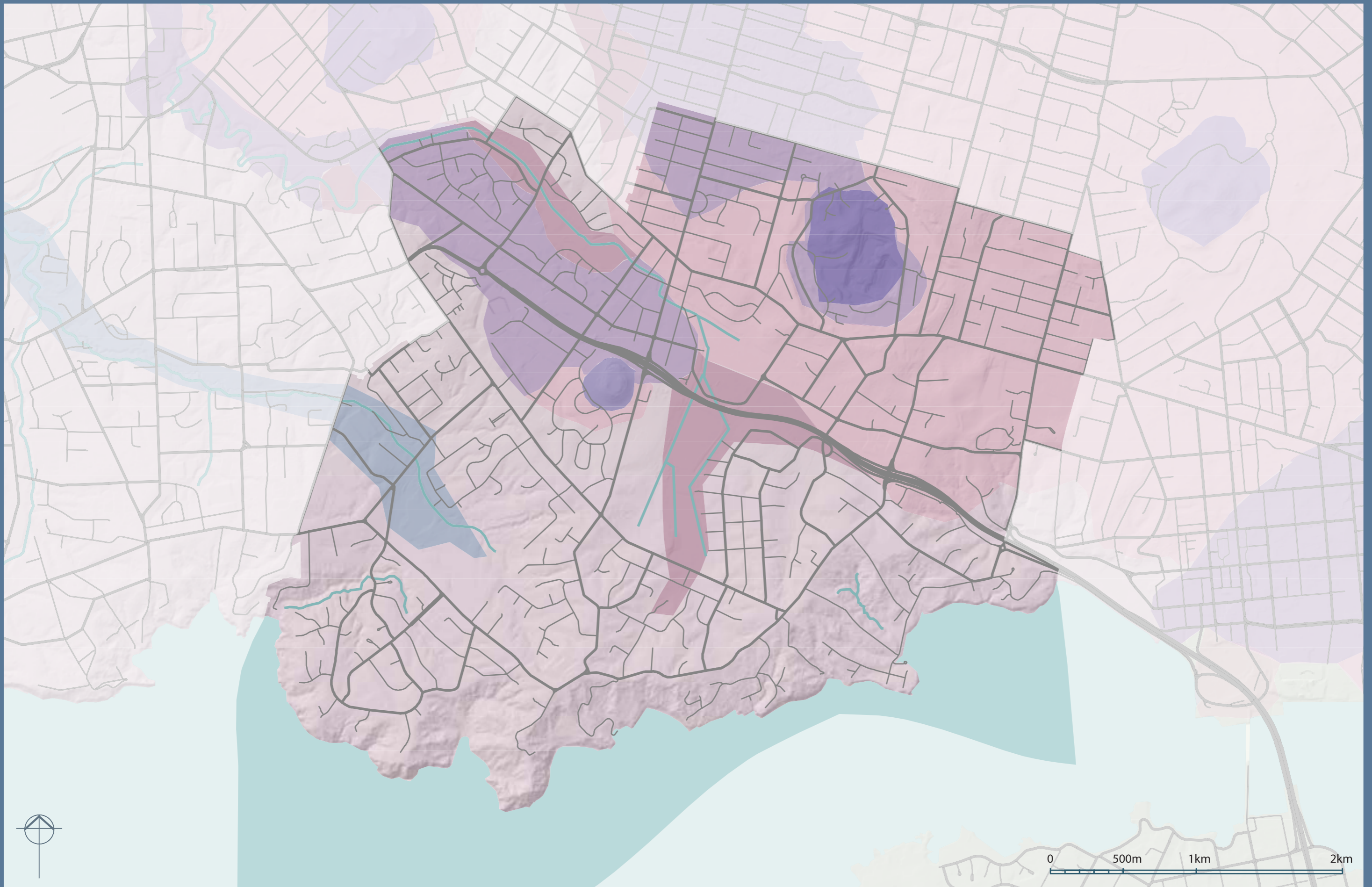
Map A1.3 - GEOMORPHOLOGY Soil/Rock Types
