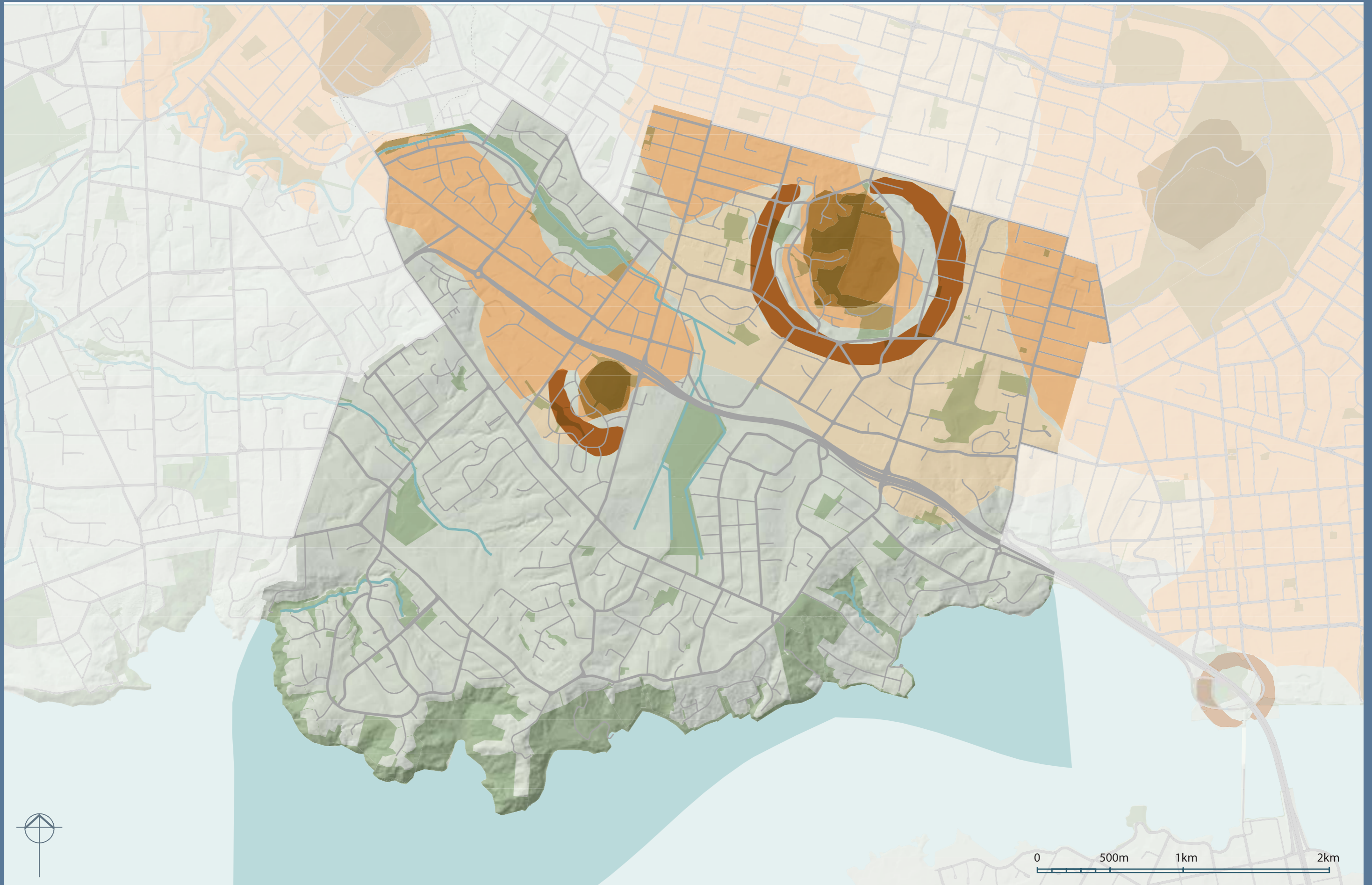
Map A1.2 - GEOMORPHOLOGY Geology
